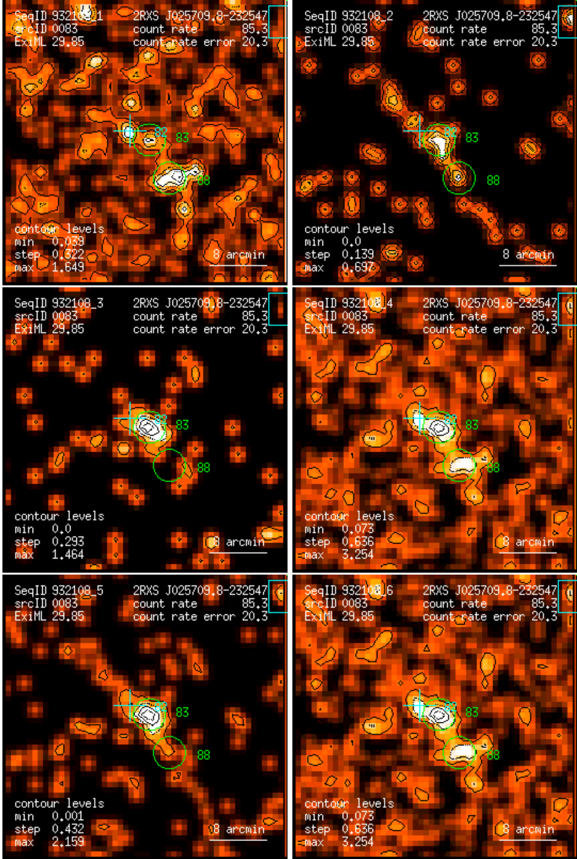
Figure 83: RASS 932108: detection 0083: band rate images, Gaussian filter: (1) PSPC channels 11 – 41, (2) 52 – 90, (3) 91 – 201, (4) 11 – 235, (5) 52 – 201, (6) 11 – 201. Broad band rates in counts/ks. Band rate contour levels in counts/ks/arcmin 2 .
