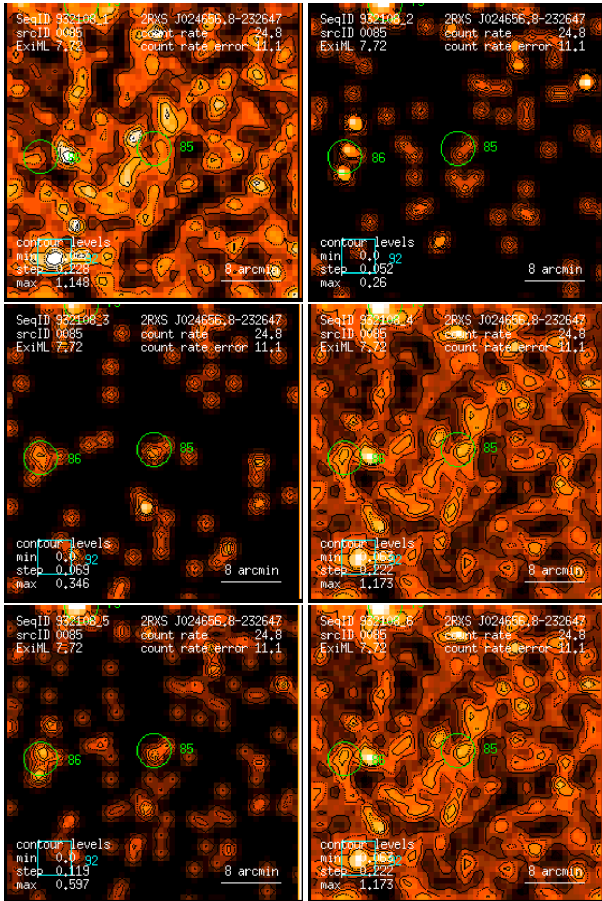
Figure 85: RASS 932108: detection 0085: band rate images, Gaussian filter: (1) PSPC channels 11 – 41, (2) 52 – 90, (3) 91 – 201, (4) 11 – 235, (5) 52 – 201, (6) 11 – 201. Broad band rates in counts/ks. Band rate contour levels in counts/ks/arcmin 2 .
