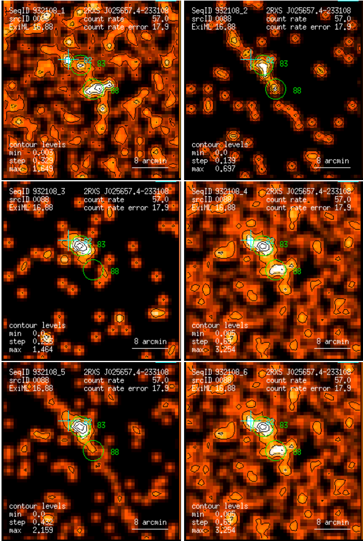
Figure 88: RASS 932108: detection 0088: band rate images, Gaussian filter: (1) PSPC channels 11 – 41, (2) 52 – 90, (3) 91 – 201, (4) 11 – 235, (5) 52 – 201, (6) 11 – 201. Broad band rates in counts/ks. Band rate contour levels in counts/ks/arcmin 2 .
