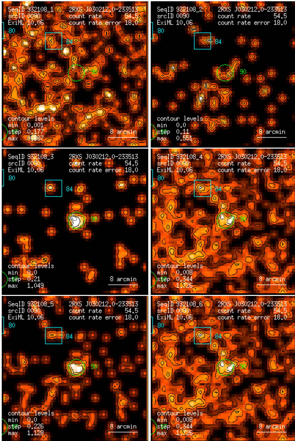
Figure 90: RASS 932108: detection 0090: band rate images, Gaussian filter: (1) PSPC channels 11 – 41, (2) 52 – 90, (3) 91 – 201, (4) 11 – 235, (5) 52 – 201, (6) 11 – 201. Broad band rates in counts/ks. Band rate contour levels in counts/ks/arcmin 2 .
