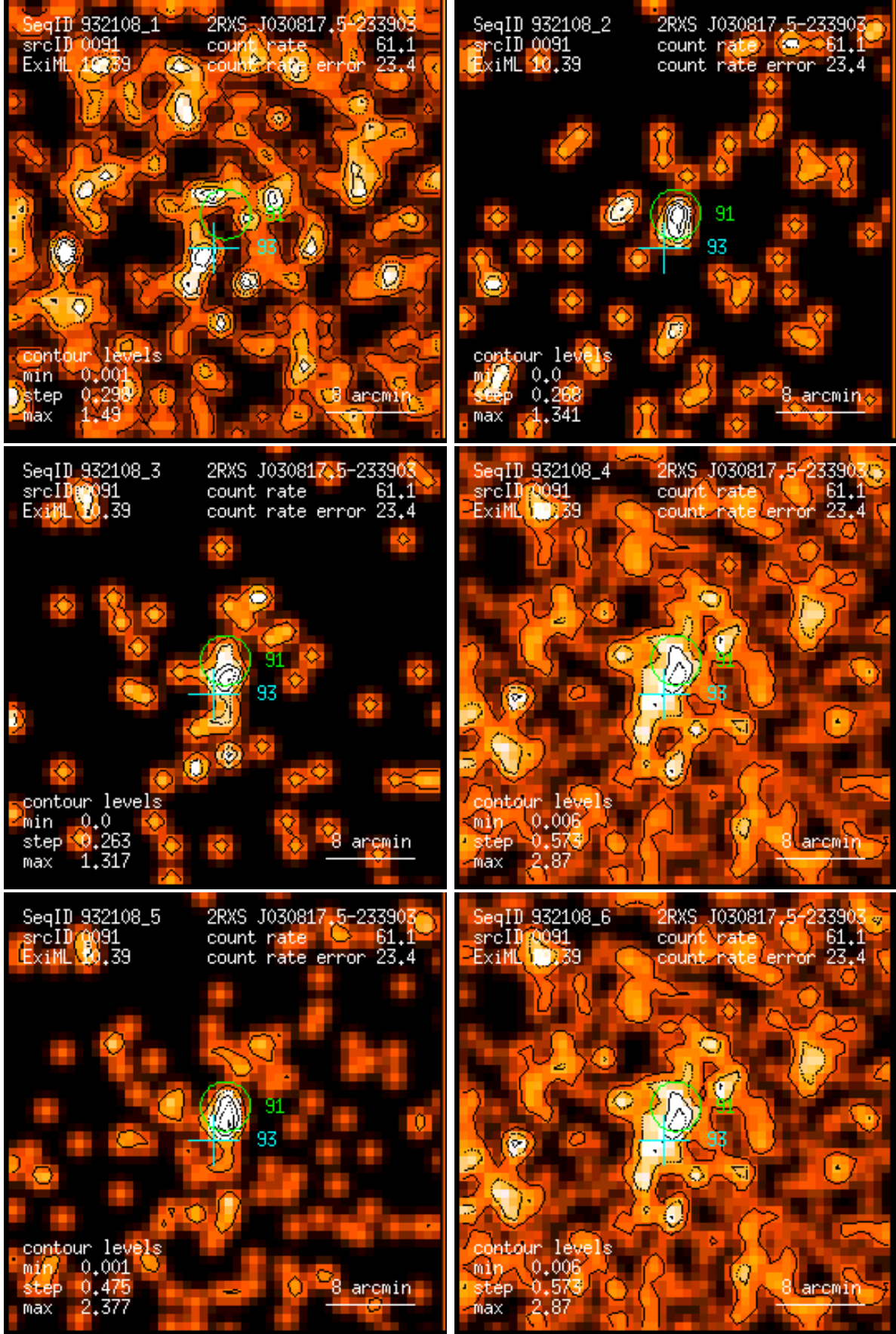
Figure 91: RASS 932108: detection 0091: band rate images, Gaussian filter: (1) PSPC channels 11 – 41, (2) 52 – 90, (3) 91 – 201, (4) 11 – 235, (5) 52 – 201, (6) 11 – 201. Broad band rates in counts/ks. Band rate contour levels in counts/ks/arcmin 2 .
