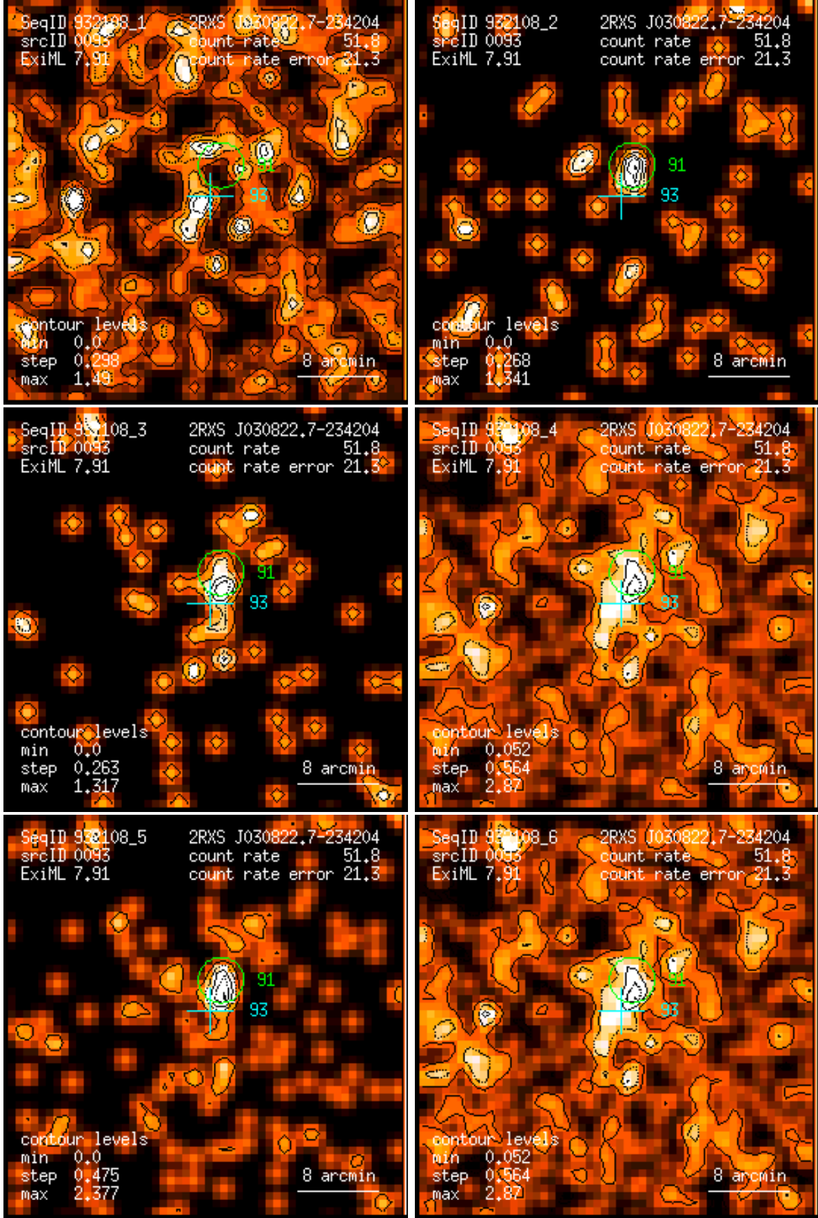
Figure 93: RASS 932108: detection 0093: band rate images, Gaussian filter: (1) PSPC channels 11 – 41, (2) 52 – 90, (3) 91 – 201, (4) 11 – 235, (5) 52 – 201, (6) 11 – 201. Broad band rates in counts/ks. Band rate contour levels in counts/ks/arcmin 2 .
