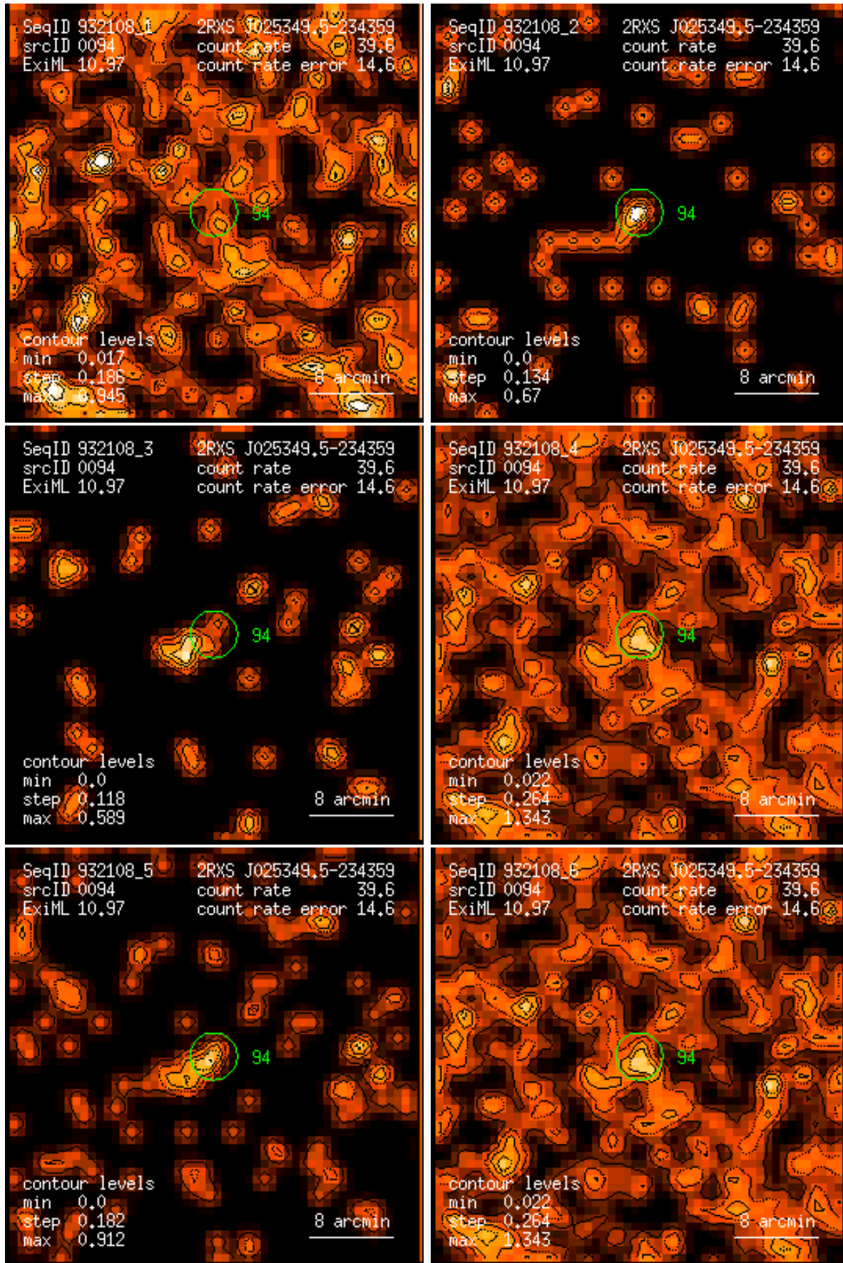
Figure 94: RASS 932108: detection 0094: band rate images, Gaussian filter: (1) PSPC channels 11 – 41, (2) 52 – 90, (3) 91 – 201, (4) 11 – 235, (5) 52 – 201, (6) 11 – 201. Broad band rates in counts/ks. Band rate contour levels in counts/ks/arcmin 2 .
