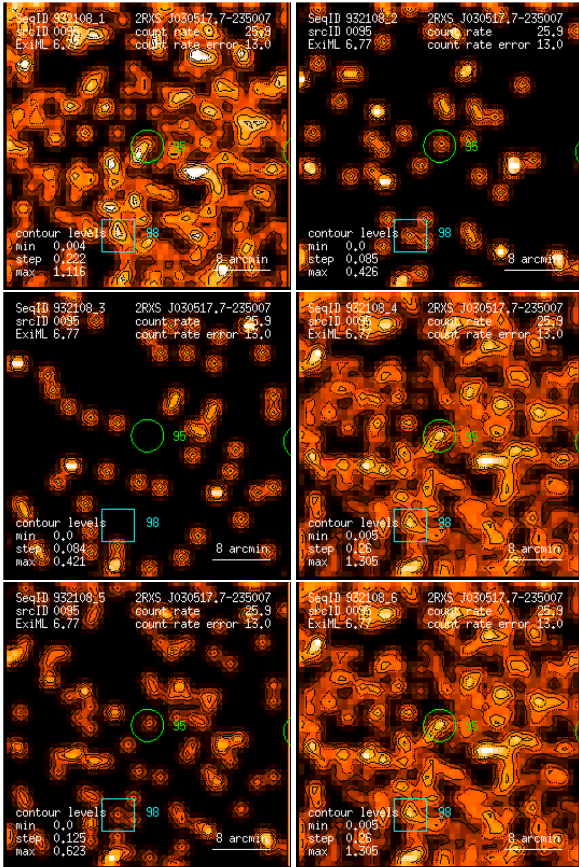
Figure 95: RASS 932108: detection 0095: band rate images, Gaussian filter: (1) PSPC channels 11 – 41, (2) 52 – 90, (3) 91 – 201, (4) 11 – 235, (5) 52 – 201, (6) 11 – 201. Broad band rates in counts/ks. Band rate contour levels in counts/ks/arcmin 2 .
