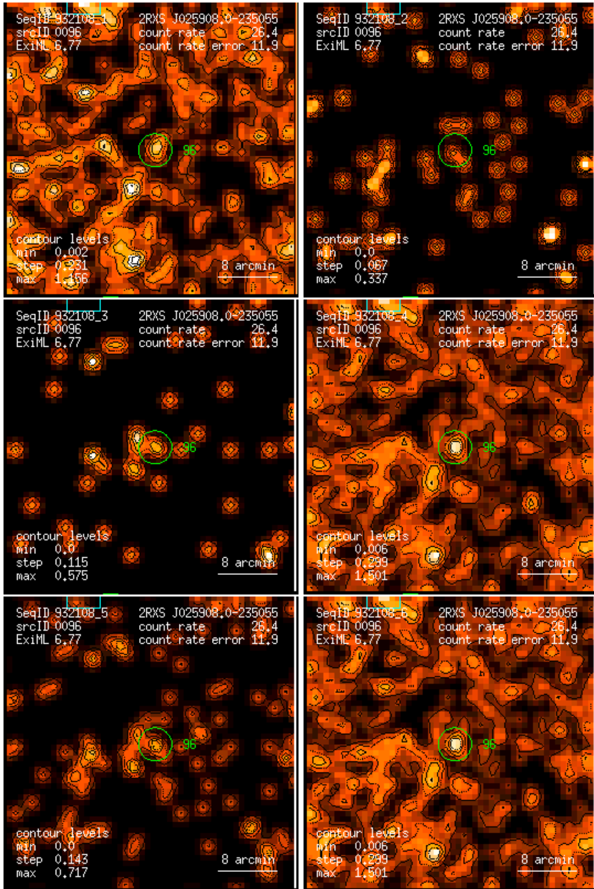
Figure 96: RASS 932108: detection 0096: band rate images, Gaussian filter: (1) PSPC channels 11 – 41, (2) 52 – 90, (3) 91 – 201, (4) 11 – 235, (5) 52 – 201, (6) 11 – 201. Broad band rates in counts/ks. Band rate contour levels in counts/ks/arcmin 2 .
