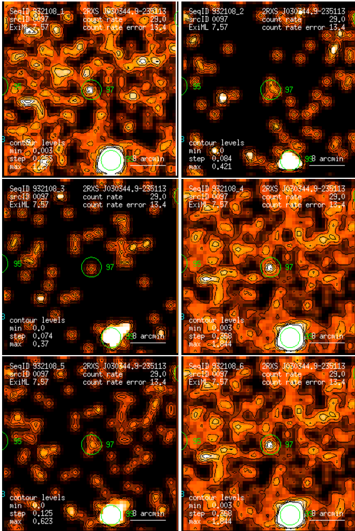
Figure 97: RASS 932108: detection 0097: band rate images, Gaussian filter: (1) PSPC channels 11 – 41, (2) 52 – 90, (3) 91 – 201, (4) 11 – 235, (5) 52 – 201, (6) 11 – 201. Broad band rates in counts/ks. Band rate contour levels in counts/ks/arcmin 2 .
