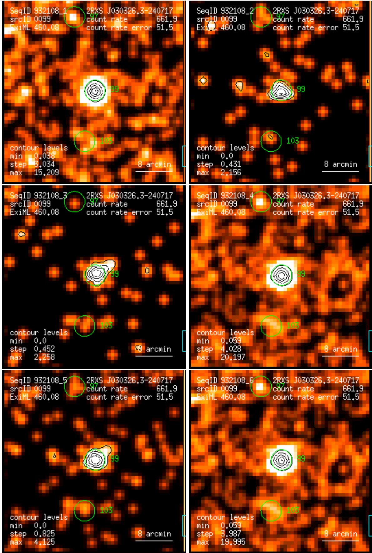
Figure 99: RASS 932108: detection 0099: band rate images, Gaussian filter: (1) PSPC channels 11 – 41, (2) 52 – 90, (3) 91 – 201, (4) 11 – 235, (5) 52 – 201, (6) 11 – 201. Broad band rates in counts/ks. Band rate contour levels in counts/ks/arcmin 2 .
