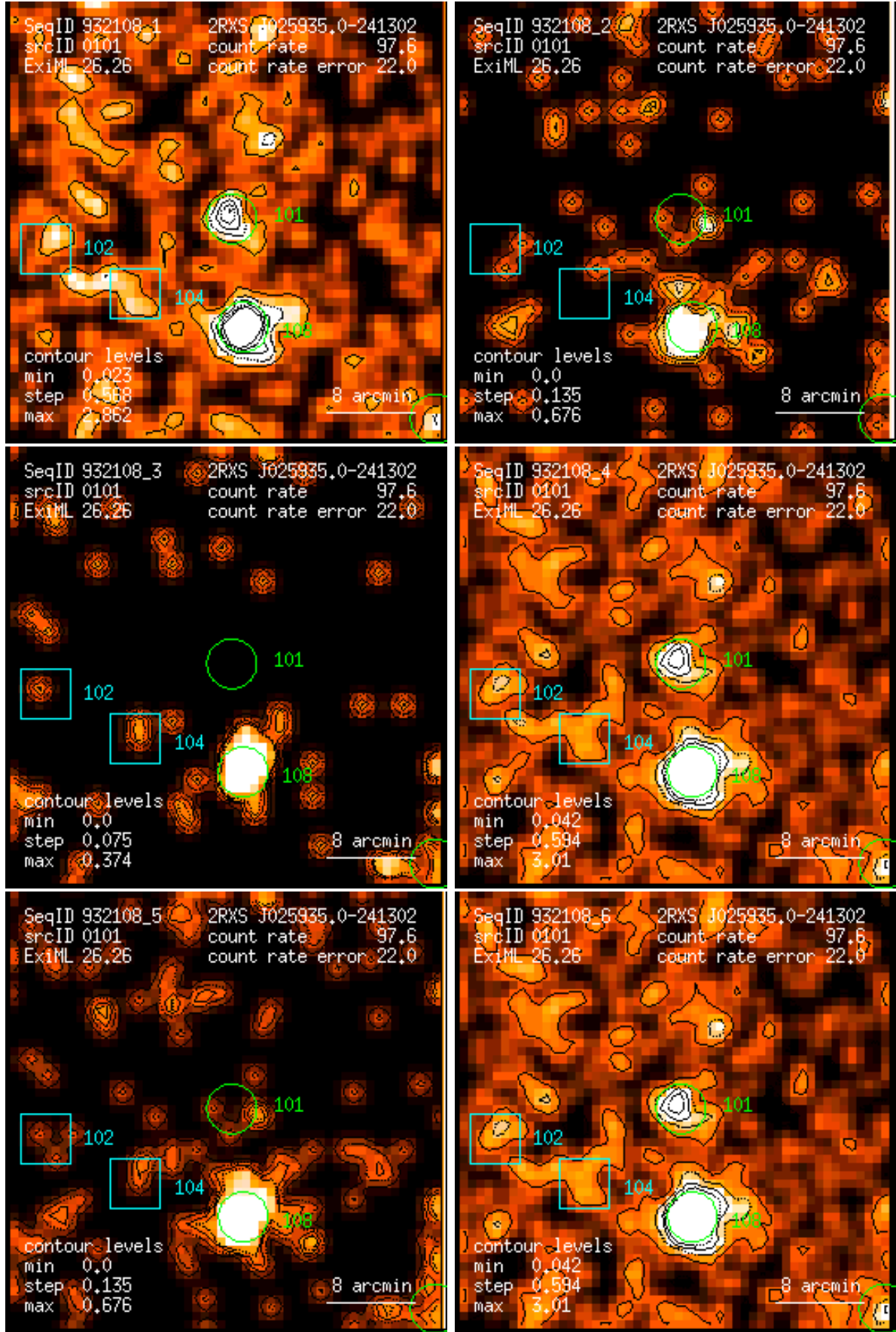
Figure 101: RASS 932108: detection 0101: band rate images, Gaussian filter: (1) PSPC channels 11 – 41, (2) 52 – 90, (3) 91 – 201, (4) 11 – 235, (5) 52 – 201, (6) 11 – 201. Broad band rates in counts/ks. Band rate contour levels in counts/ks/arcmin 2 .
