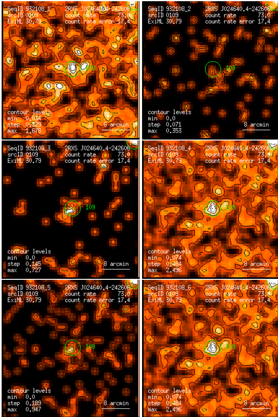
Figure 109: RASS 932108: detection 0109: band rate images, Gaussian filter: (1) PSPC channels 11 – 41, (2) 52 – 90, (3) 91 – 201, (4) 11 – 235, (5) 52 – 201, (6) 11 – 201. Broad band rates in counts/ks. Band rate contour levels in counts/ks/arcmin 2 .
