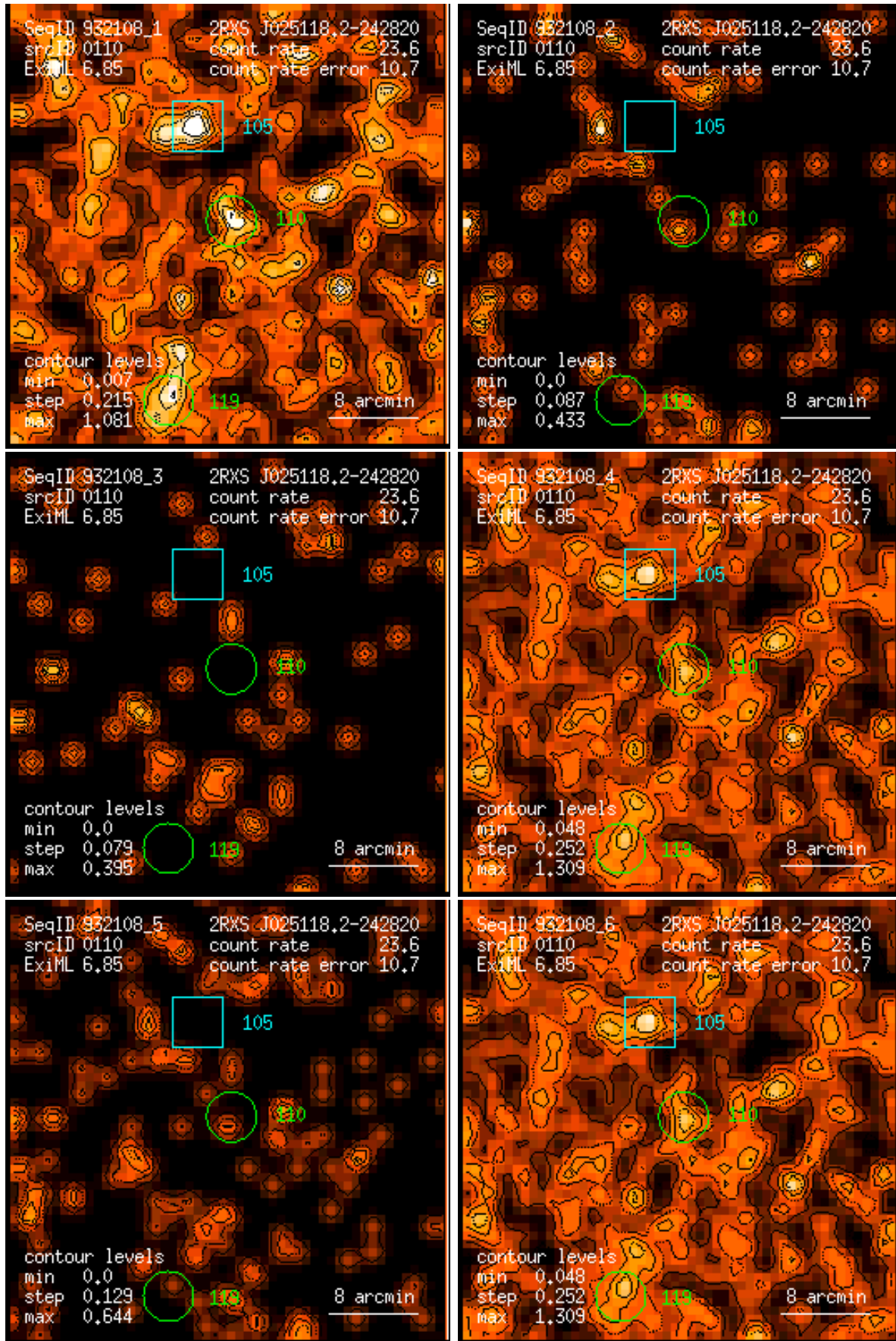
Figure 110: RASS 932108: detection 0110: band rate images, Gaussian filter: (1) PSPC channels 11 – 41, (2) 52 – 90, (3) 91 – 201, (4) 11 – 235, (5) 52 – 201, (6) 11 – 201. Broad band rates in counts/ks. Band rate contour levels in counts/ks/arcmin 2 .
