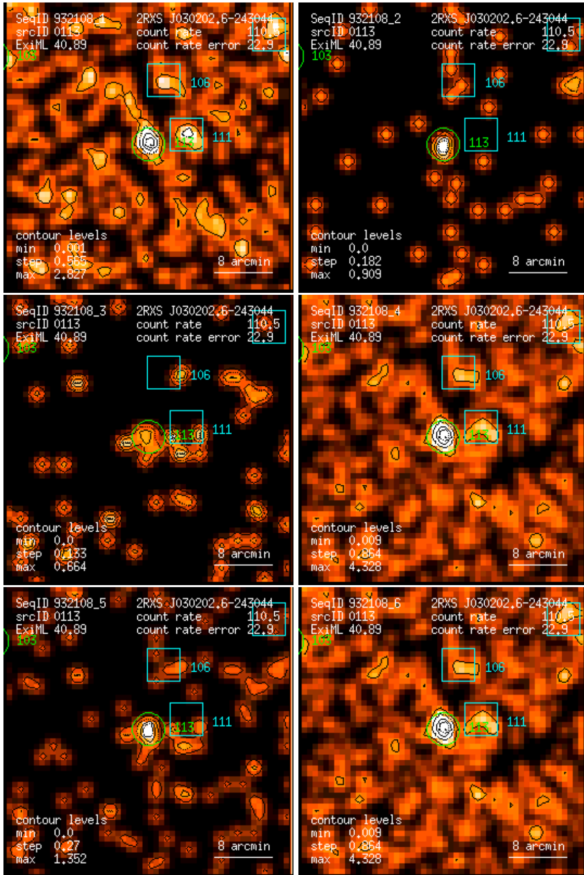
Figure 113: RASS 932108: detection 0113: band rate images, Gaussian filter: (1) PSPC channels 11 – 41, (2) 52 – 90, (3) 91 – 201, (4) 11 – 235, (5) 52 – 201, (6) 11 – 201. Broad band rates in counts/ks. Band rate contour levels in counts/ks/arcmin 2 .
