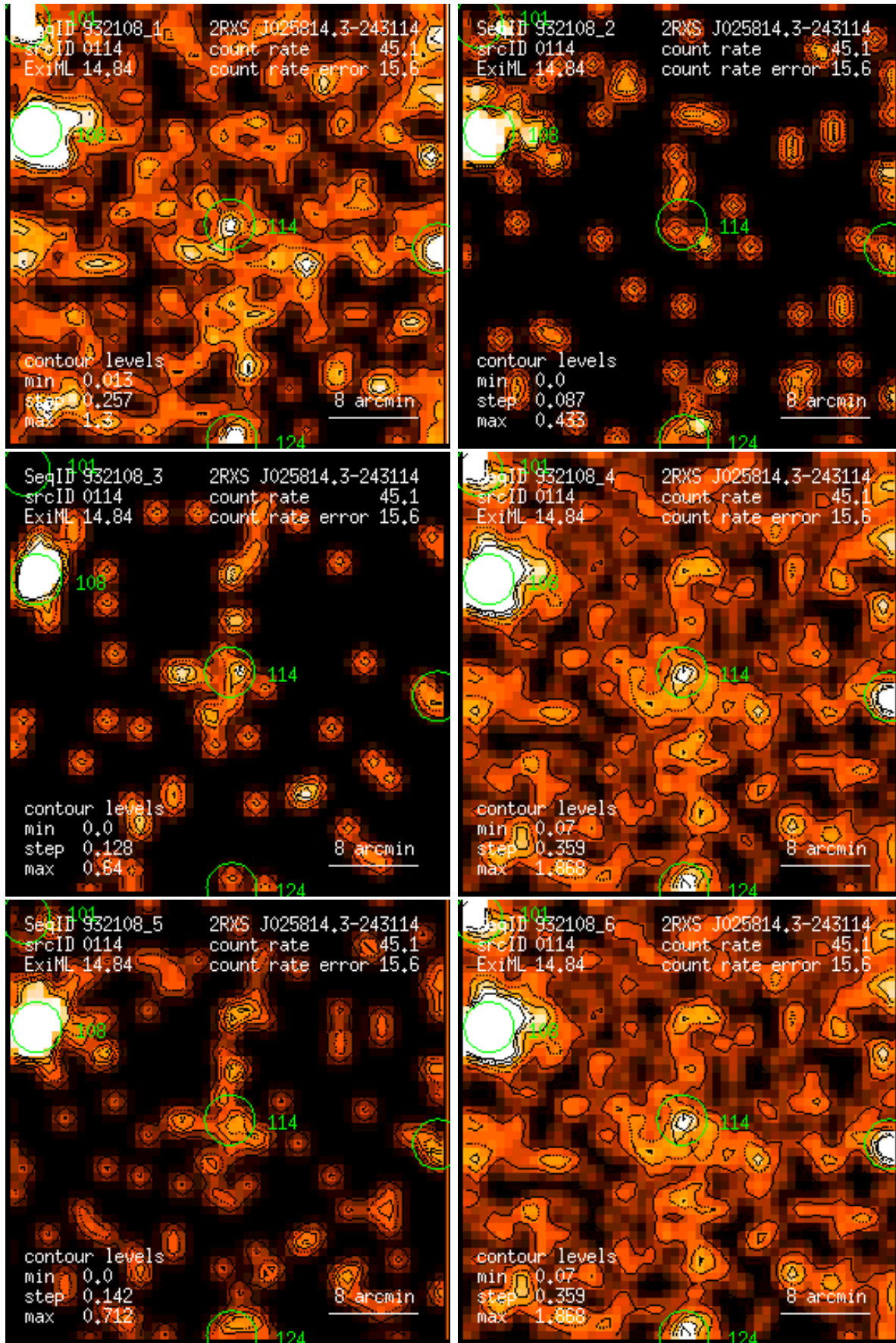
Figure 114: RASS 932108: detection 0114: band rate images, Gaussian filter: (1) PSPC channels 11 – 41, (2) 52 – 90, (3) 91 – 201, (4) 11 – 235, (5) 52 – 201, (6) 11 – 201. Broad band rates in counts/ks. Band rate contour levels in counts/ks/arcmin 2 .
