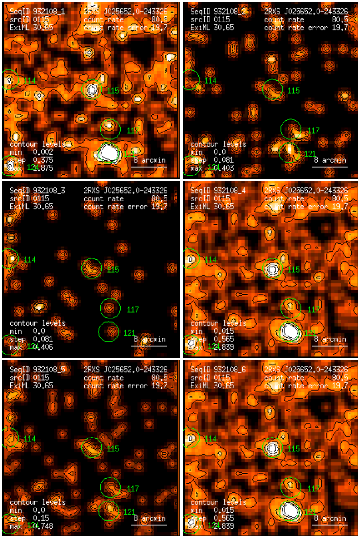
Figure 115: RASS 932108: detection 0115: band rate images, Gaussian filter: (1) PSPC channels 11 – 41, (2) 52 – 90, (3) 91 – 201, (4) 11 – 235, (5) 52 – 201, (6) 11 – 201. Broad band rates in counts/ks. Band rate contour levels in counts/ks/arcmin 2 .
