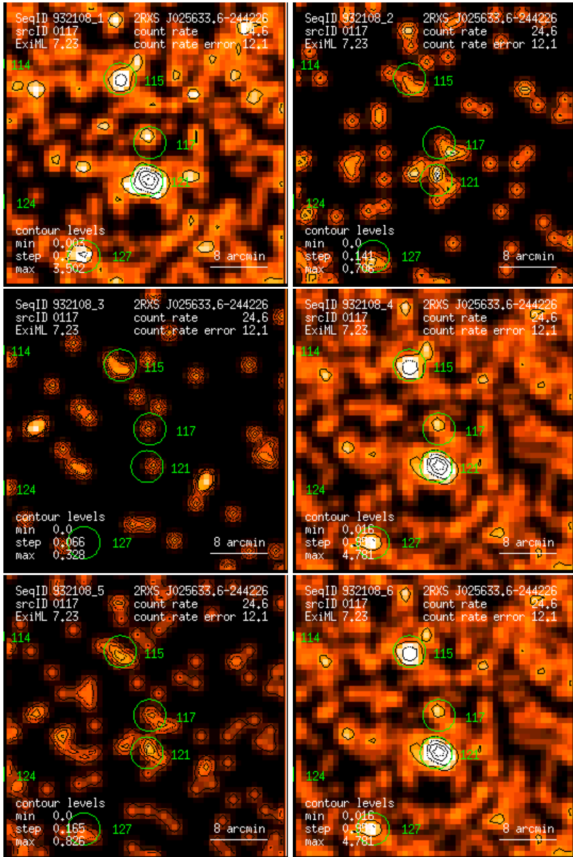
Figure 117: RASS 932108: detection 0117: band rate images, Gaussian filter: (1) PSPC channels 11 – 41, (2) 52 – 90, (3) 91 – 201, (4) 11 – 235, (5) 52 – 201, (6) 11 – 201. Broad band rates in counts/ks. Band rate contour levels in counts/ks/arcmin 2 .
