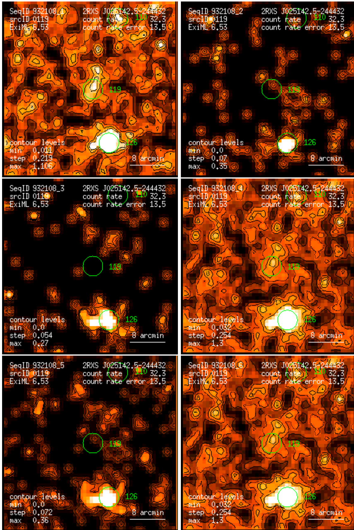
Figure 119: RASS 932108: detection 0119: band rate images, Gaussian filter: (1) PSPC channels 11 – 41, (2) 52 – 90, (3) 91 – 201, (4) 11 – 235, (5) 52 – 201, (6) 11 – 201. Broad band rates in counts/ks. Band rate contour levels in counts/ks/arcmin 2 .
