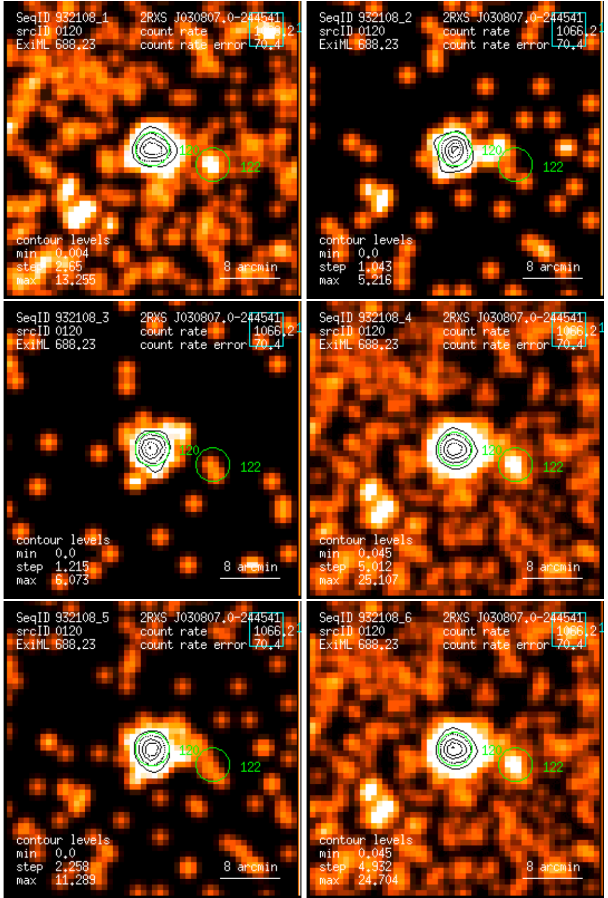
Figure 120: RASS 932108: detection 0120: band rate images, Gaussian filter: (1) PSPC channels 11 – 41, (2) 52 – 90, (3) 91 – 201, (4) 11 – 235, (5) 52 – 201, (6) 11 – 201. Broad band rates in counts/ks. Band rate contour levels in counts/ks/arcmin 2 .
