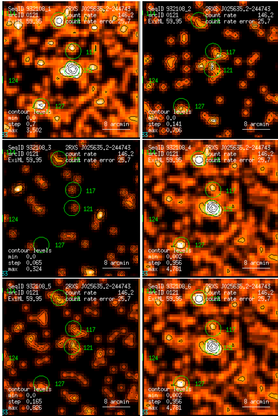
Figure 121: RASS 932108: detection 0121: band rate images, Gaussian filter: (1) PSPC channels 11 – 41, (2) 52 – 90, (3) 91 – 201, (4) 11 – 235, (5) 52 – 201, (6) 11 – 201. Broad band rates in counts/ks. Band rate contour levels in counts/ks/arcmin 2 .
