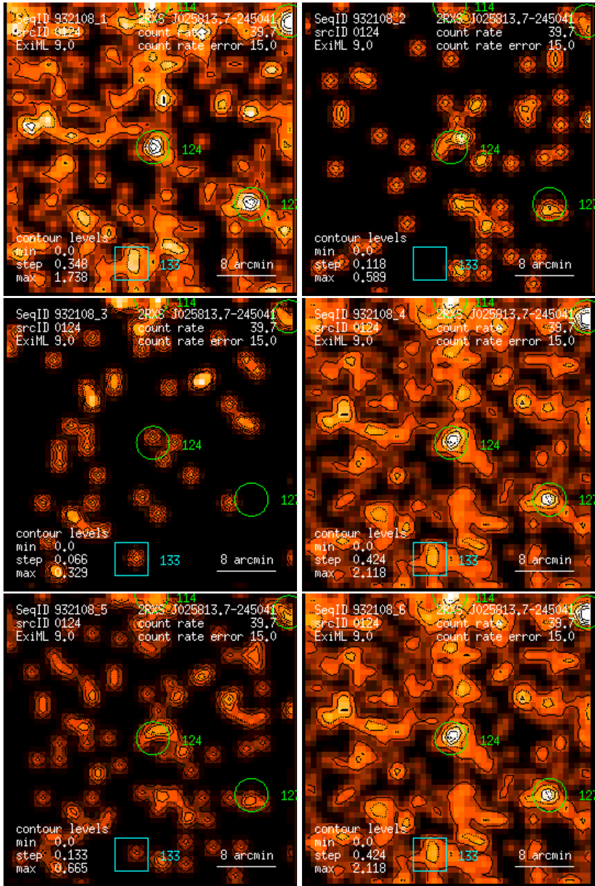
Figure 124: RASS 932108: detection 0124: band rate images, Gaussian filter: (1) PSPC channels 11 – 41, (2) 52 – 90, (3) 91 – 201, (4) 11 – 235, (5) 52 – 201, (6) 11 – 201. Broad band rates in counts/ks. Band rate contour levels in counts/ks/arcmin 2 .
