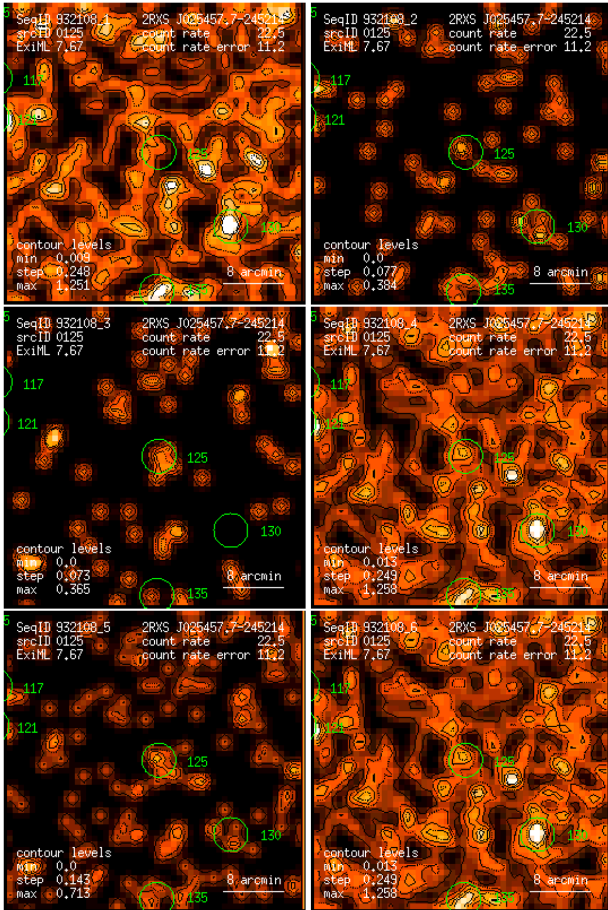
Figure 125: RASS 932108: detection 0125: band rate images, Gaussian filter: (1) PSPC channels 11 – 41, (2) 52 – 90, (3) 91 – 201, (4) 11 – 235, (5) 52 – 201, (6) 11 – 201. Broad band rates in counts/ks. Band rate contour levels in counts/ks/arcmin 2 .
