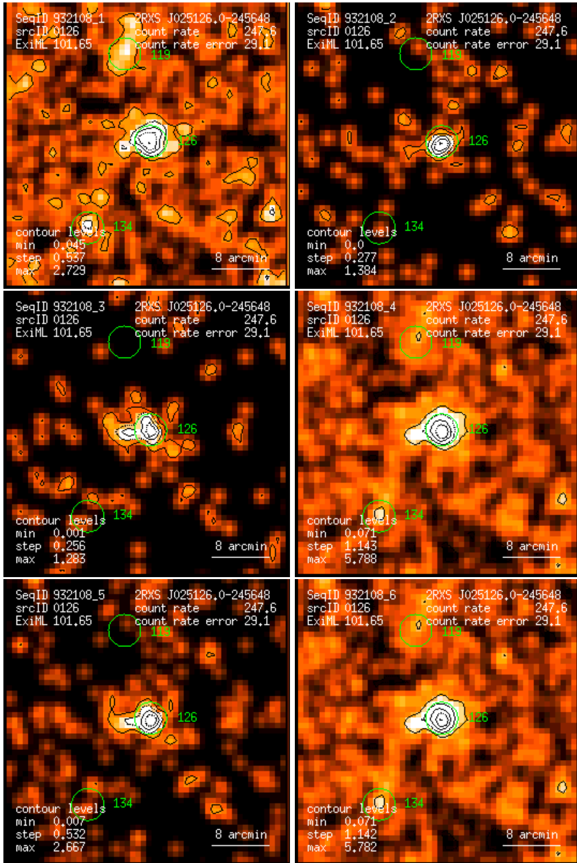
Figure 126: RASS 932108: detection 0126: band rate images, Gaussian filter: (1) PSPC channels 11 – 41, (2) 52 – 90, (3) 91 – 201, (4) 11 – 235, (5) 52 – 201, (6) 11 – 201. Broad band rates in counts/ks. Band rate contour levels in counts/ks/arcmin 2 .
