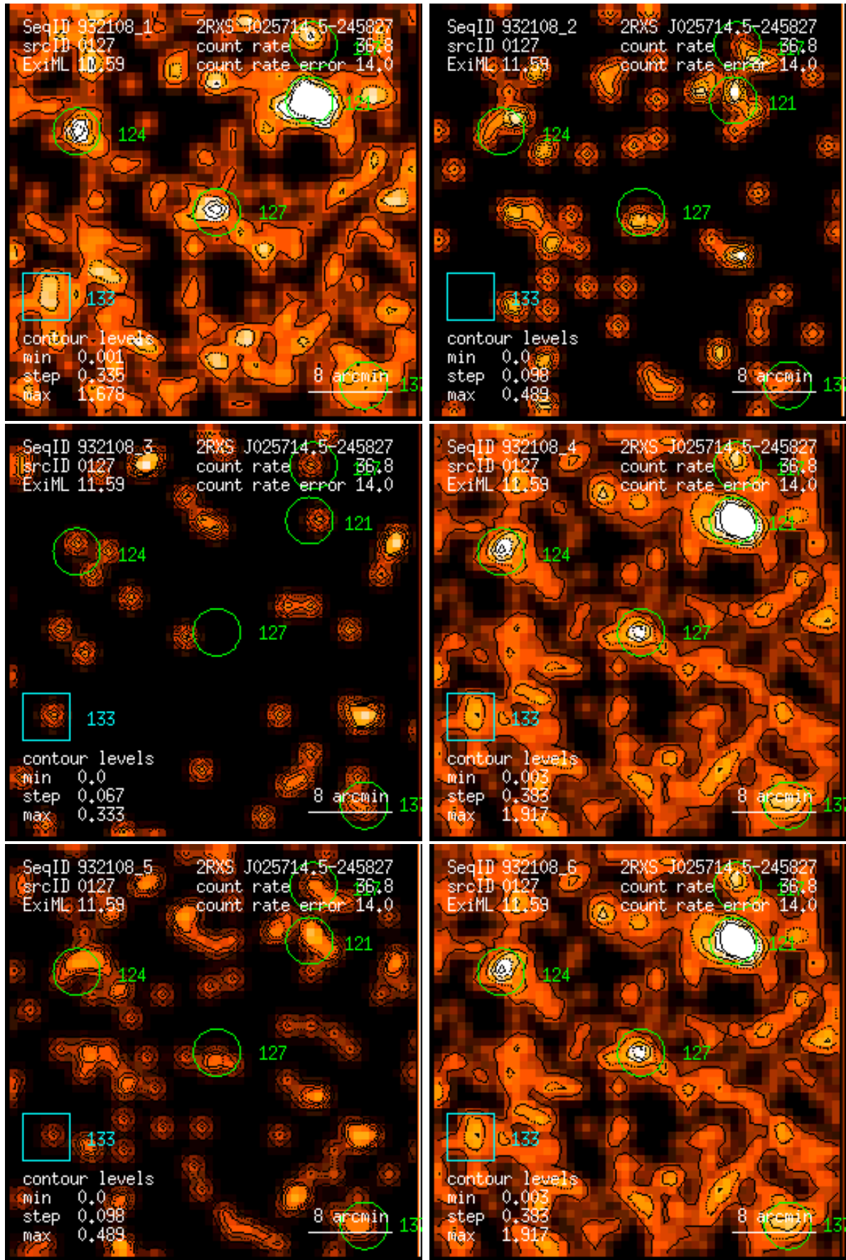
Figure 127: RASS 932108: detection 0127: band rate images, Gaussian filter: (1) PSPC channels 11 – 41, (2) 52 – 90, (3) 91 – 201, (4) 11 – 235, (5) 52 – 201, (6) 11 – 201. Broad band rates in counts/ks. Band rate contour levels in counts/ks/arcmin 2 .
