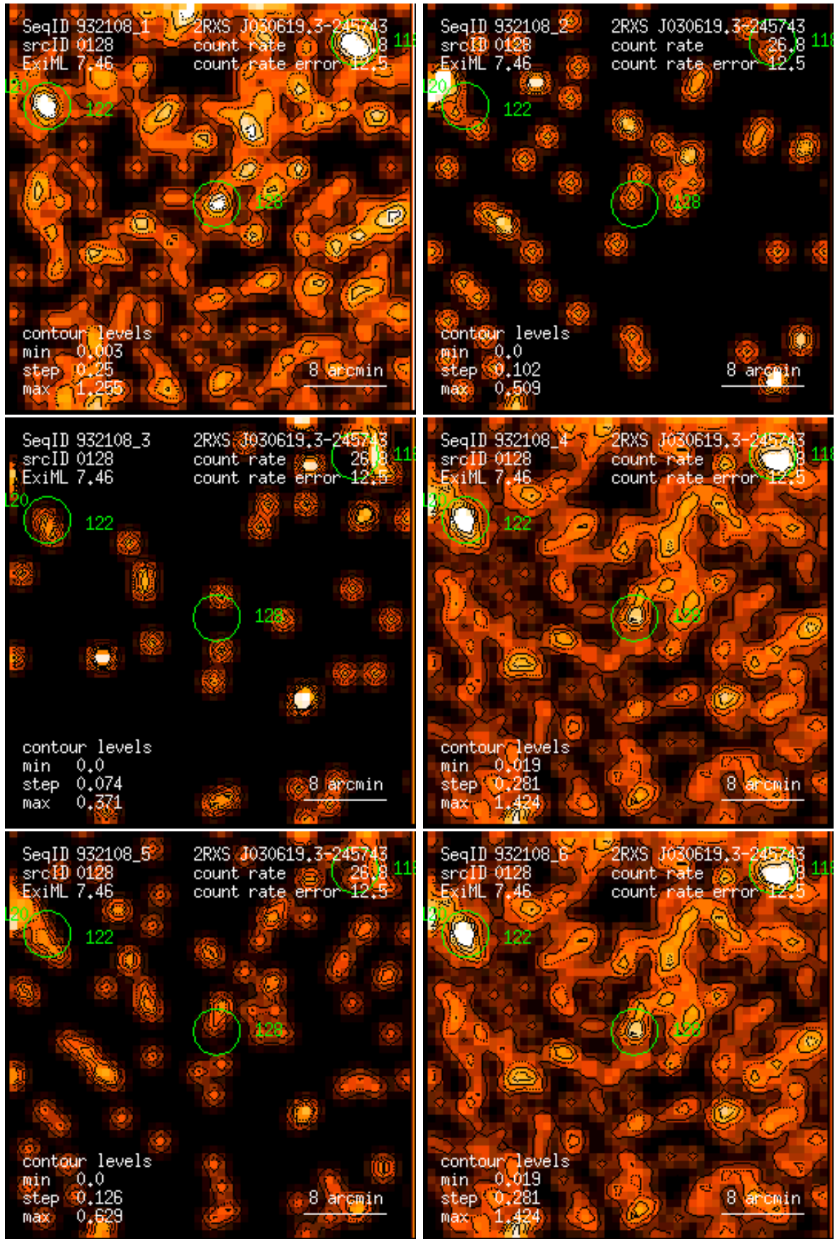
Figure 128: RASS 932108: detection 0128: band rate images, Gaussian filter: (1) PSPC channels 11 – 41, (2) 52 – 90, (3) 91 – 201, (4) 11 – 235, (5) 52 – 201, (6) 11 – 201. Broad band rates in counts/ks. Band rate contour levels in counts/ks/arcmin 2 .
