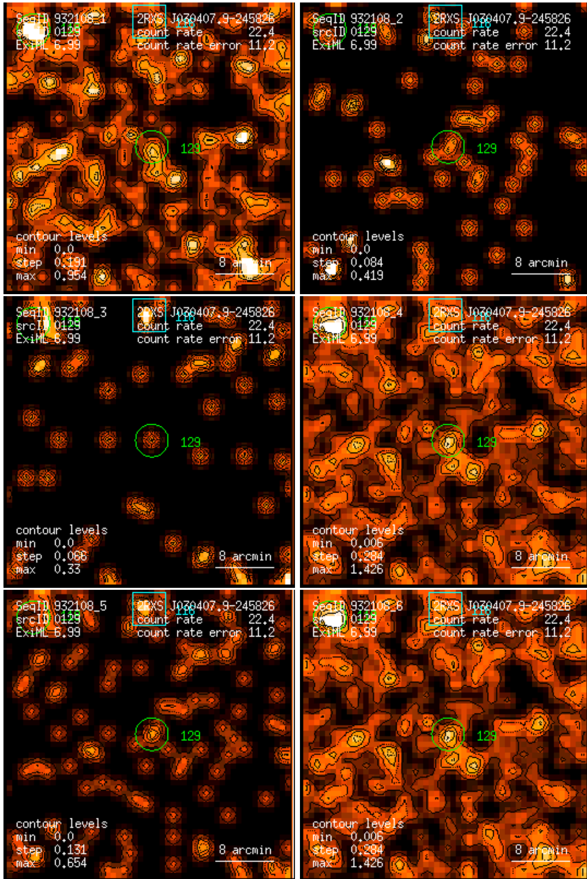
Figure 129: RASS 932108: detection 0129: band rate images, Gaussian filter: (1) PSPC channels 11 – 41, (2) 52 – 90, (3) 91 – 201, (4) 11 – 235, (5) 52 – 201, (6) 11 – 201. Broad band rates in counts/ks. Band rate contour levels in counts/ks/arcmin 2 .
