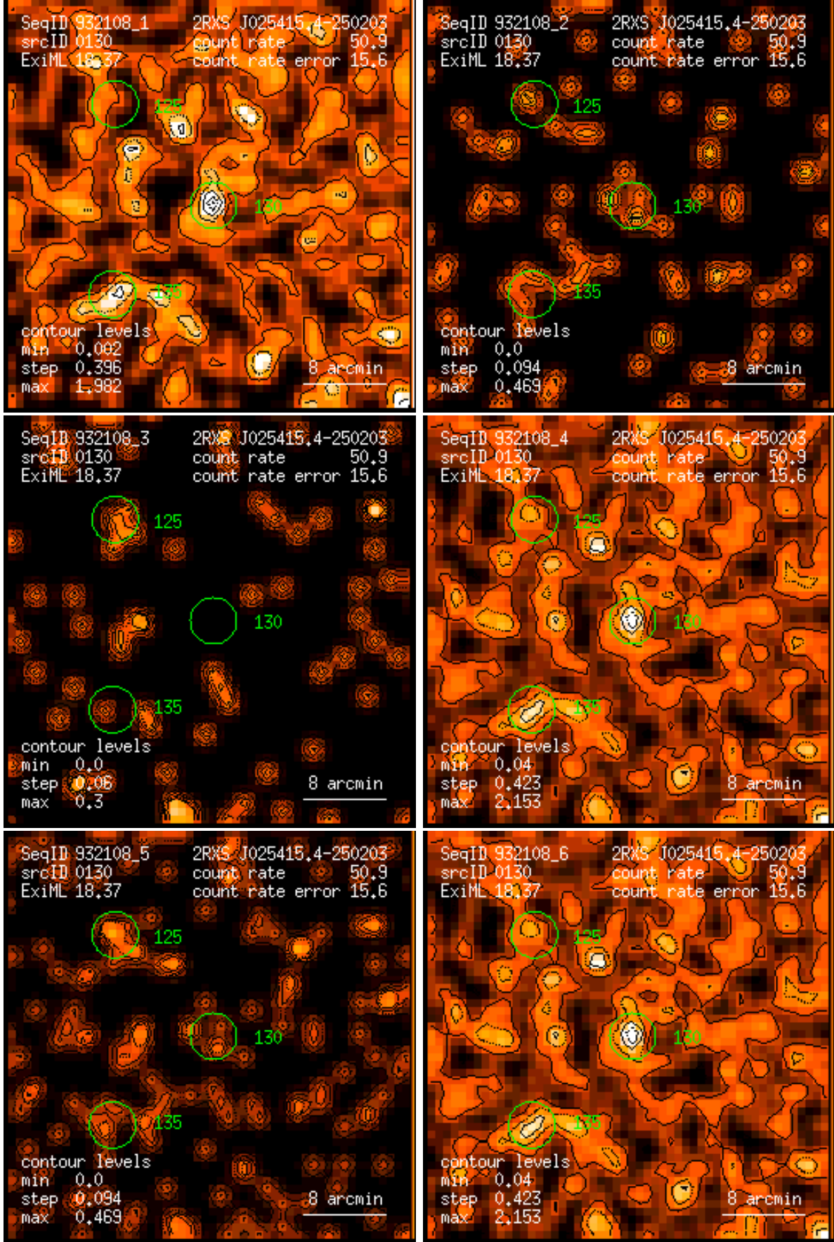
Figure 130: RASS 932108: detection 0130: band rate images, Gaussian filter: (1) PSPC channels 11 – 41, (2) 52 – 90, (3) 91 – 201, (4) 11 – 235, (5) 52 – 201, (6) 11 – 201. Broad band rates in counts/ks. Band rate contour levels in counts/ks/arcmin 2 .
