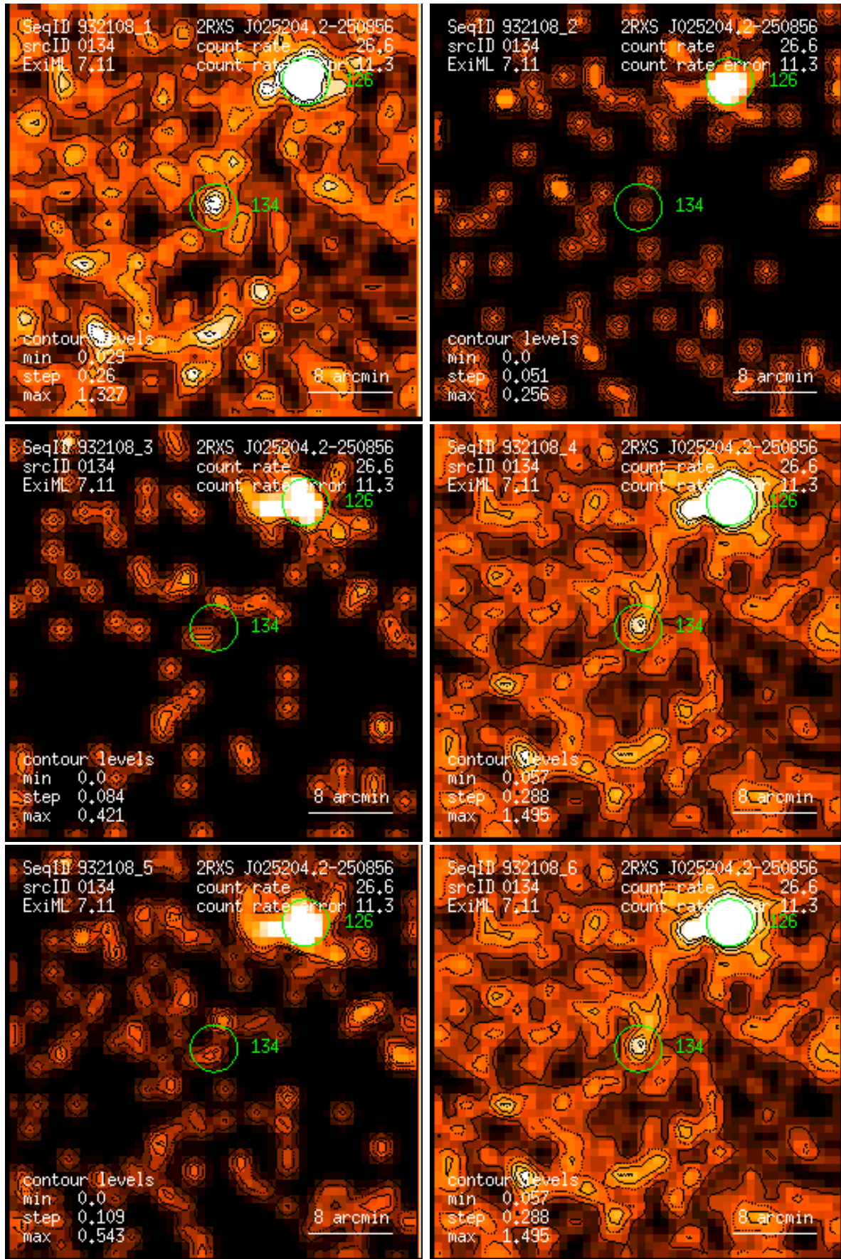
Figure 134: RASS 932108: detection 0134: band rate images, Gaussian filter: (1) PSPC channels 11 – 41, (2) 52 – 90, (3) 91 – 201, (4) 11 – 235, (5) 52 – 201, (6) 11 – 201. Broad band rates in counts/ks. Band rate contour levels in counts/ks/arcmin 2 .
