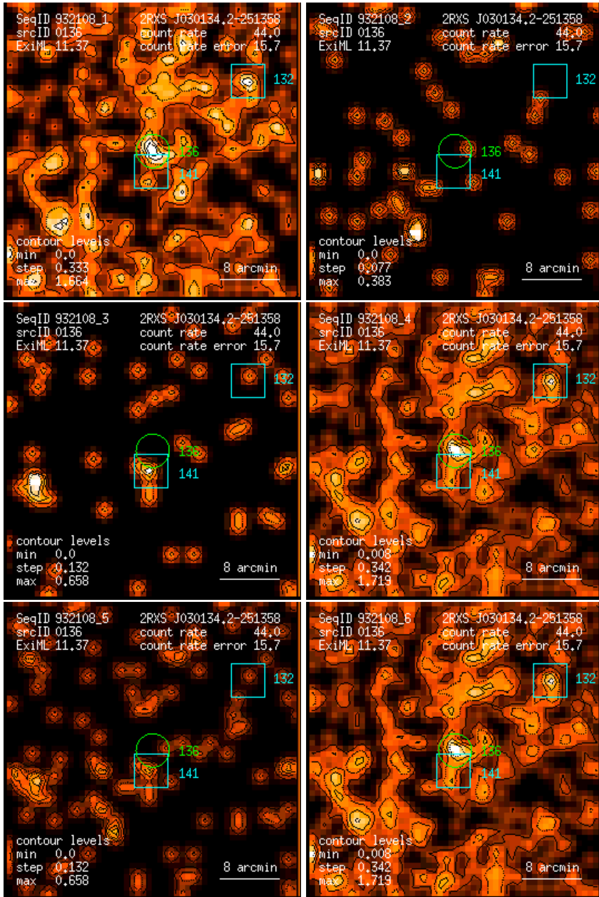
Figure 136: RASS 932108: detection 0136: band rate images, Gaussian filter: (1) PSPC channels 11 – 41, (2) 52 – 90, (3) 91 – 201, (4) 11 – 235, (5) 52 – 201, (6) 11 – 201. Broad band rates in counts/ks. Band rate contour levels in counts/ks/arcmin 2 .
