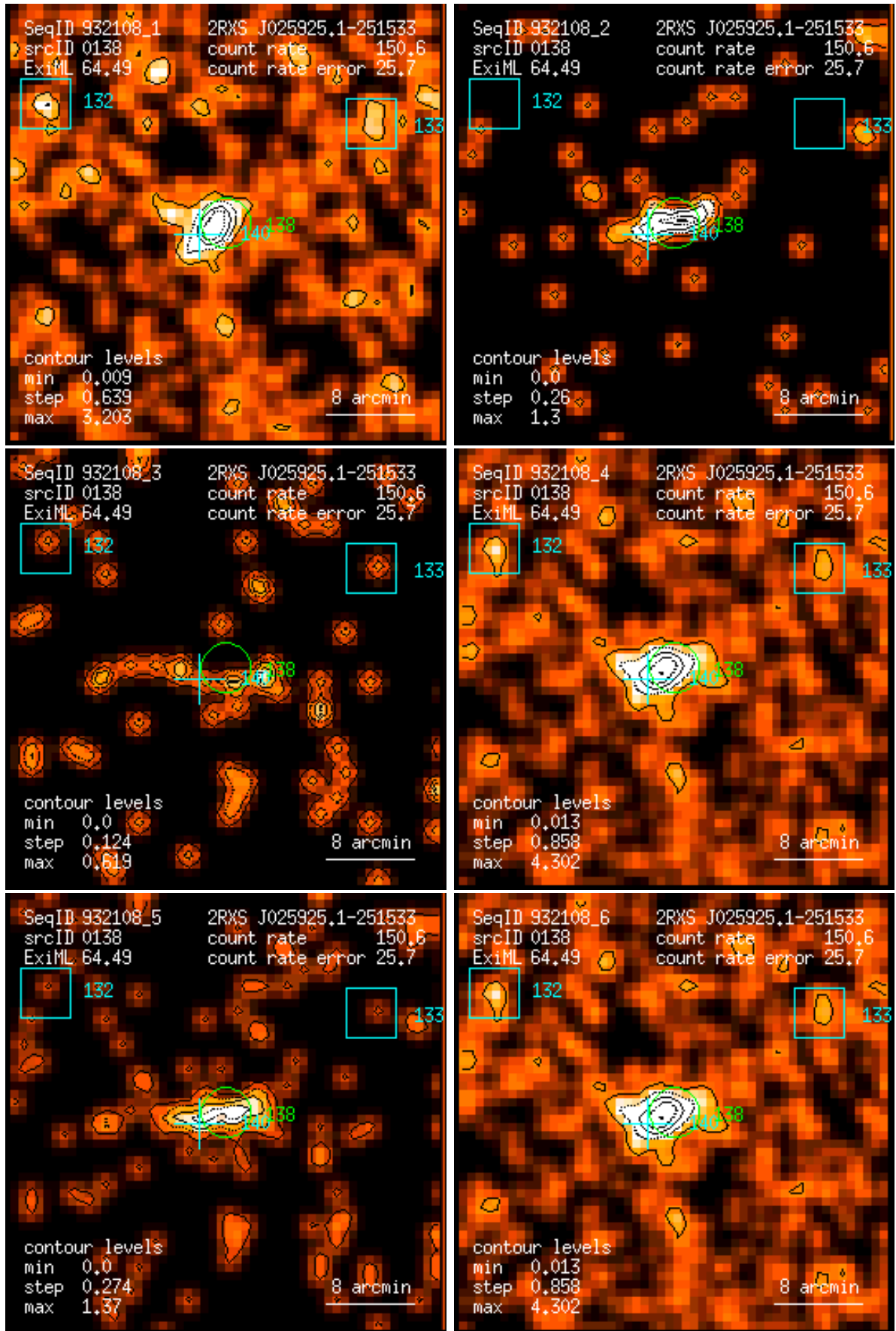
Figure 138: RASS 932108: detection 0138: band rate images, Gaussian filter: (1) PSPC channels 11 – 41, (2) 52 – 90, (3) 91 – 201, (4) 11 – 235, (5) 52 – 201, (6) 11 – 201. Broad band rates in counts/ks. Band rate contour levels in counts/ks/arcmin 2 .
