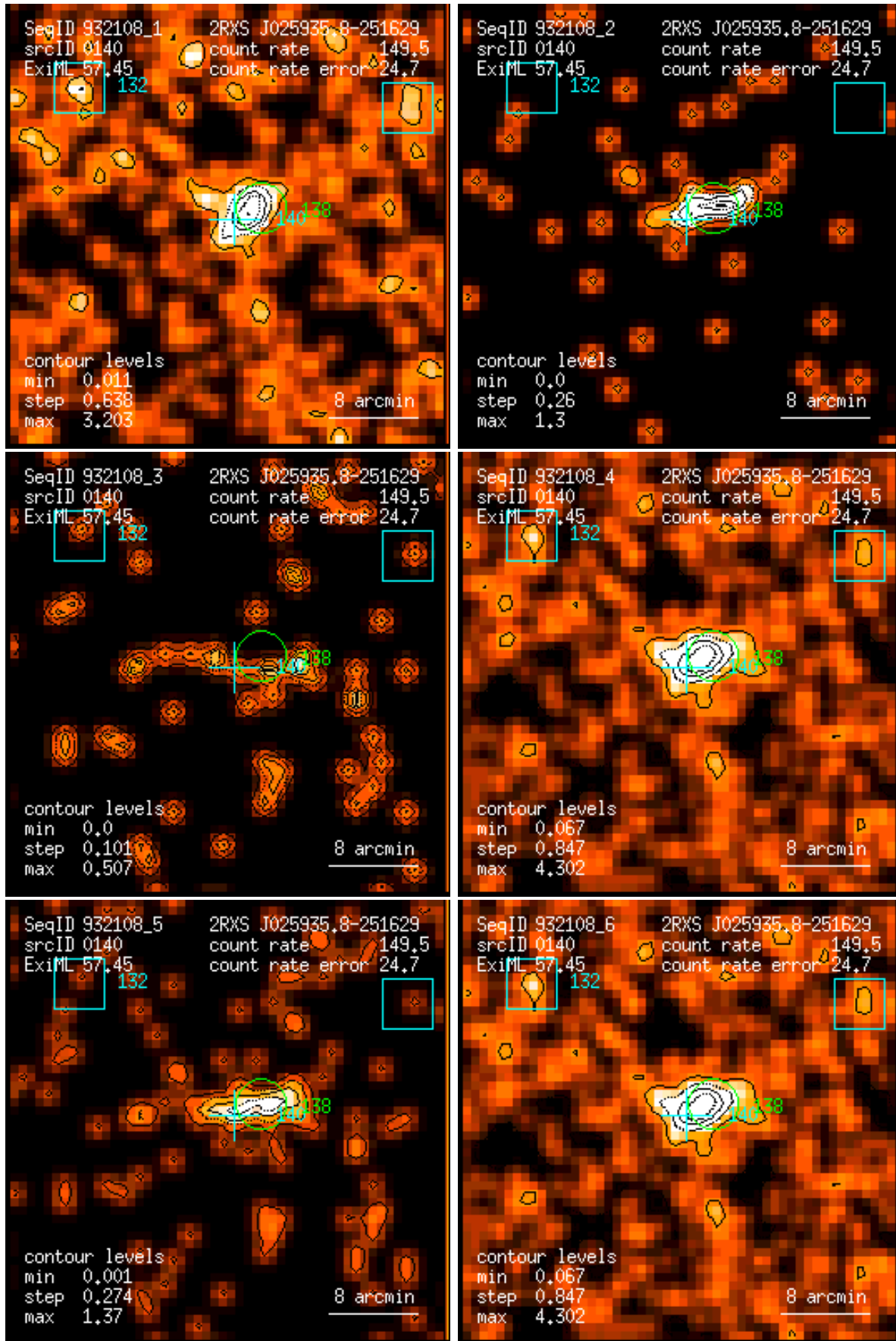
Figure 140: RASS 932108: detection 0140: band rate images, Gaussian filter: (1) PSPC channels 11 – 41, (2) 52 – 90, (3) 91 – 201, (4) 11 – 235, (5) 52 – 201, (6) 11 – 201. Broad band rates in counts/ks. Band rate contour levels in counts/ks/arcmin 2 .
