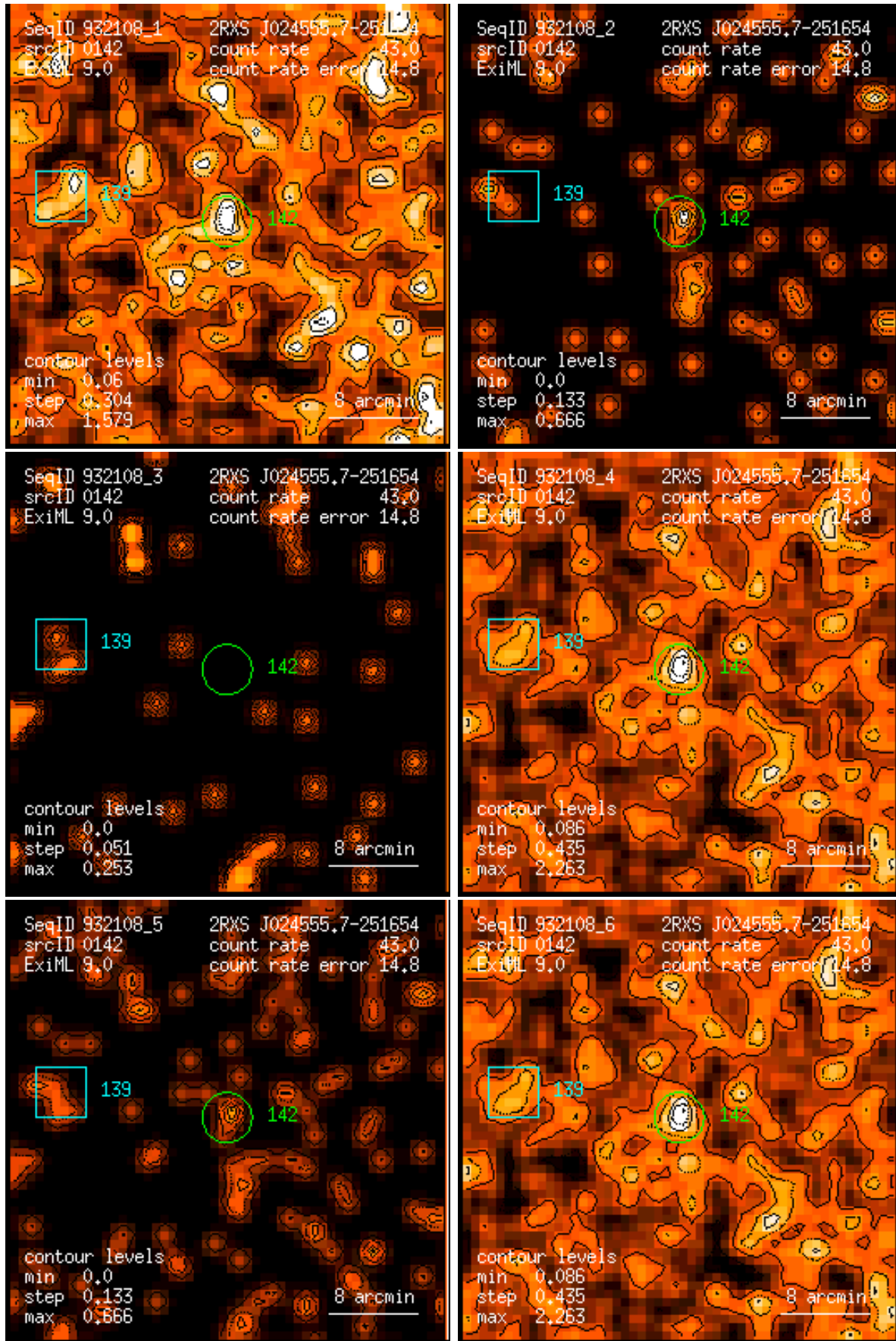
Figure 142: RASS 932108: detection 0142: band rate images, Gaussian filter: (1) PSPC channels 11 – 41, (2) 52 – 90, (3) 91 – 201, (4) 11 – 235, (5) 52 – 201, (6) 11 – 201. Broad band rates in counts/ks. Band rate contour levels in counts/ks/arcmin 2 .
