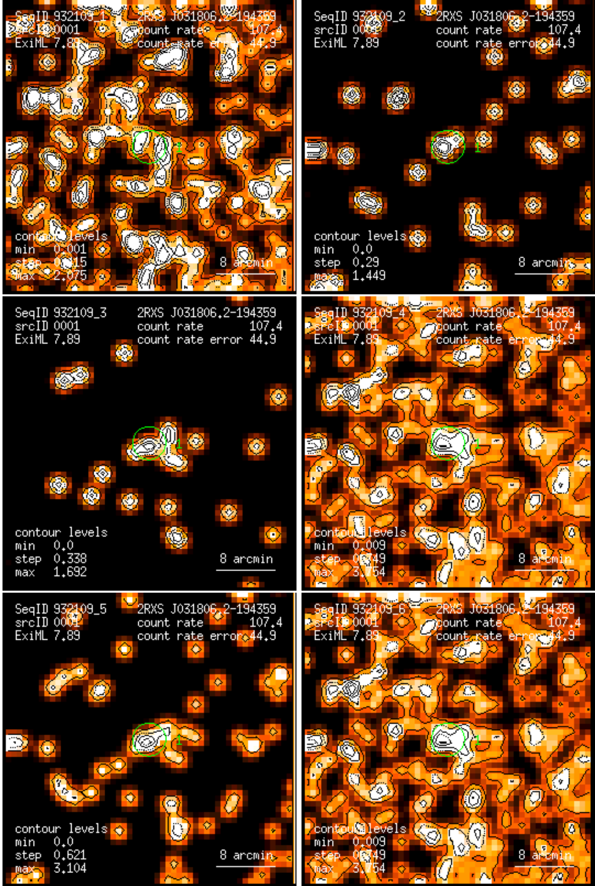
Figure 1: RASS 932109: detection 0001: band rate images, Gaussian filter: (1) PSPC channels 11 – 41, (2) 52 – 90, (3) 91 – 201, (4) 11 – 235, (5) 52 – 201, (6) 11 – 201. Broad band rates in counts/ks. Band rate contour levels in counts/ks/arcmin 2 .
