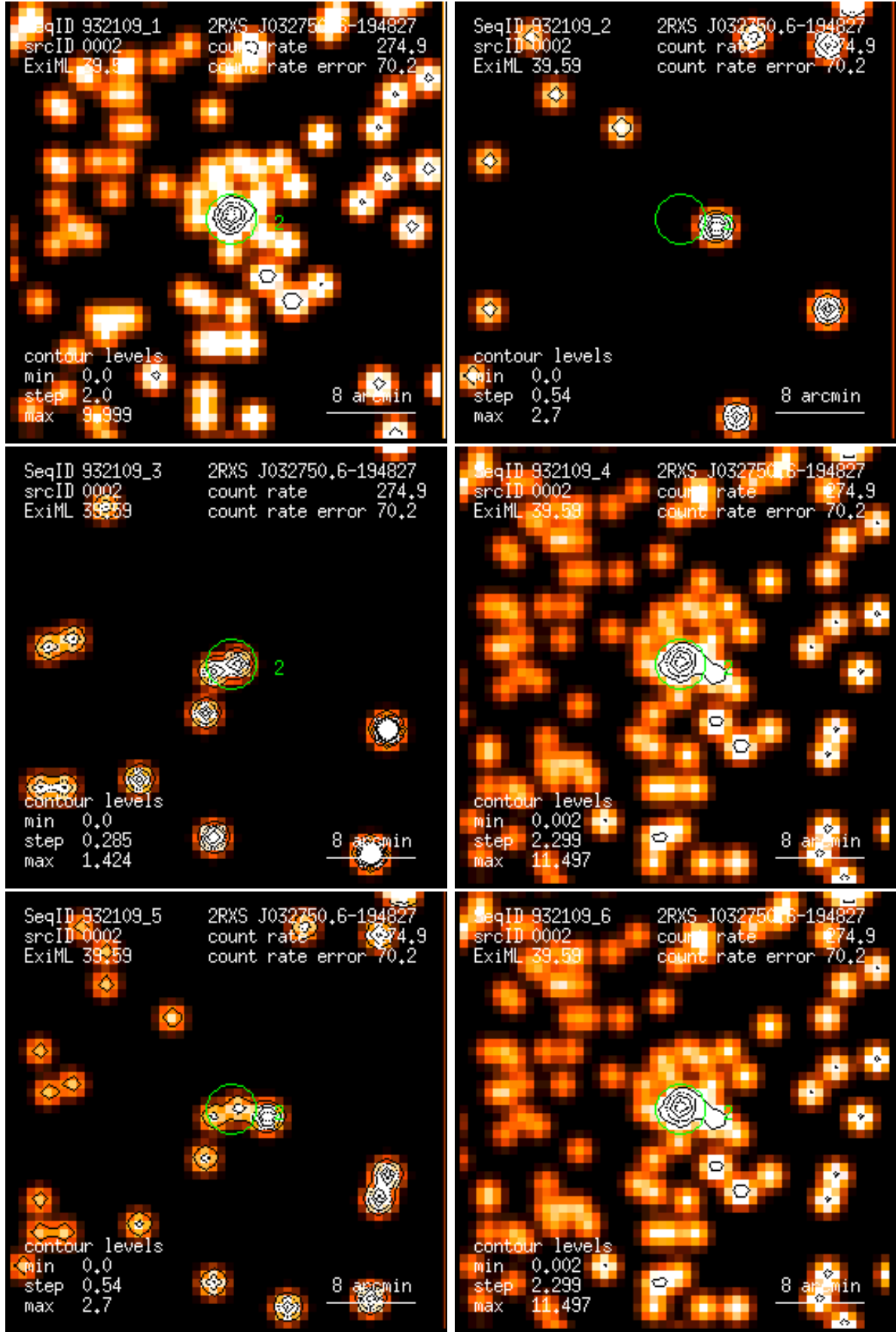
Figure 2: RASS 932109: detection 0002: band rate images, Gaussian filter: (1) PSPC channels 11 – 41, (2) 52 – 90, (3) 91 – 201, (4) 11 – 235, (5) 52 – 201, (6) 11 – 201. Broad band rates in counts/ks. Band rate contour levels in counts/ks/arcmin 2 .
