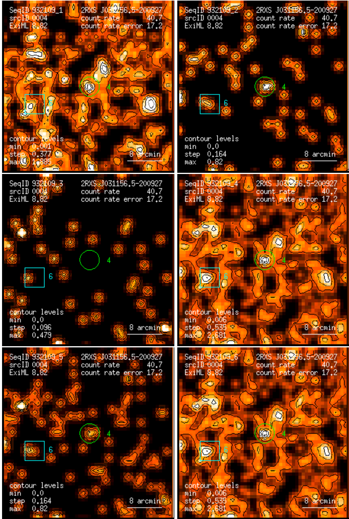
Figure 4: RASS 932109: detection 0004: band rate images, Gaussian filter: (1) PSPC channels 11 – 41, (2) 52 – 90, (3) 91 – 201, (4) 11 – 235, (5) 52 – 201, (6) 11 – 201. Broad band rates in counts/ks. Band rate contour levels in counts/ks/arcmin 2 .
