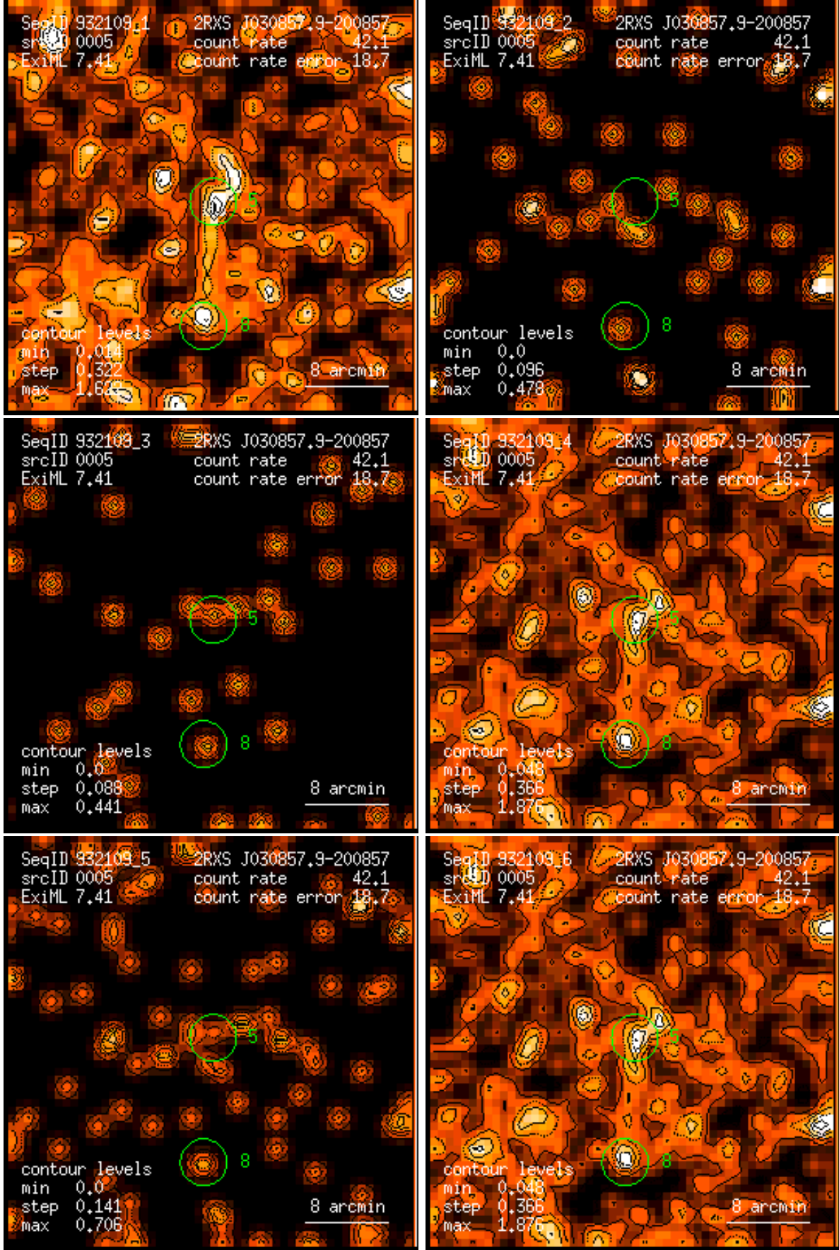
Figure 5: RASS 932109: detection 0005: band rate images, Gaussian filter: (1) PSPC channels 11 – 41, (2) 52 – 90, (3) 91 – 201, (4) 11 – 235, (5) 52 – 201, (6) 11 – 201. Broad band rates in counts/ks. Band rate contour levels in counts/ks/arcmin 2 .
