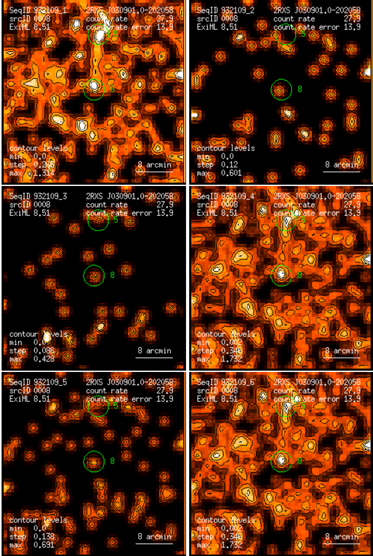
Figure 8: RASS 932109: detection 0008: band rate images, Gaussian filter: (1) PSPC channels 11 – 41, (2) 52 – 90, (3) 91 – 201, (4) 11 – 235, (5) 52 – 201, (6) 11 – 201. Broad band rates in counts/ks. Band rate contour levels in counts/ks/arcmin 2 .
