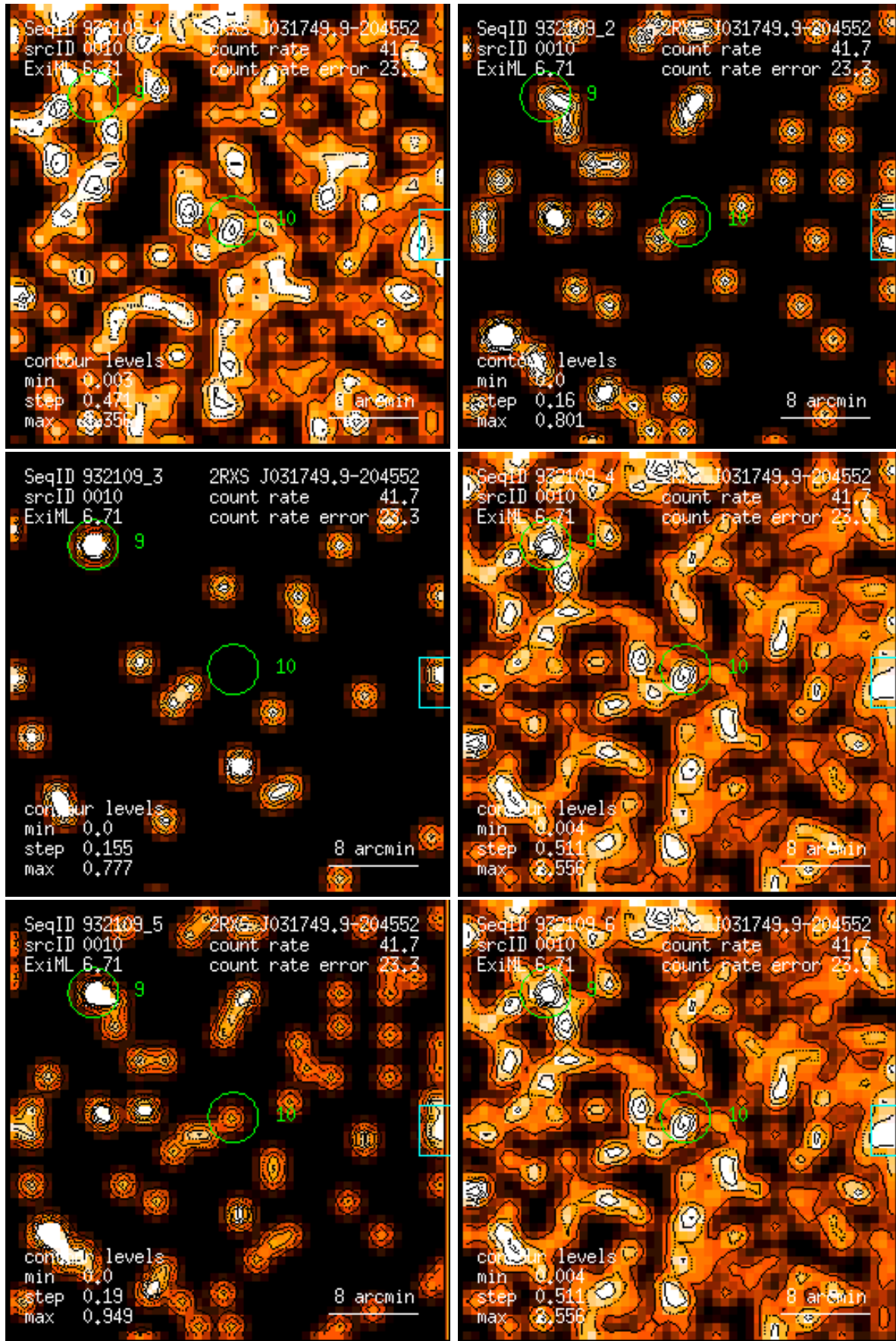
Figure 10: RASS 932109: detection 0010: band rate images, Gaussian filter: (1) PSPC channels 11 – 41, (2) 52 – 90, (3) 91 – 201, (4) 11 – 235, (5) 52 – 201, (6) 11 – 201. Broad band rates in counts/ks. Band rate contour levels in counts/ks/arcmin 2 .
