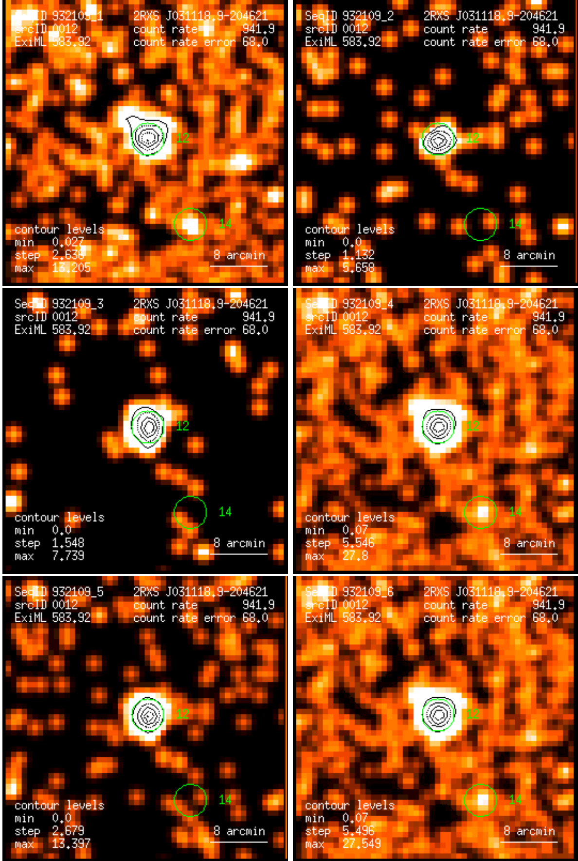
Figure 12: RASS 932109: detection 0012: band rate images, Gaussian filter: (1) PSPC channels 11 – 41, (2) 52 – 90, (3) 91 – 201, (4) 11 – 235, (5) 52 – 201, (6) 11 – 201. Broad band rates in counts/ks. Band rate contour levels in counts/ks/arcmin 2 .
