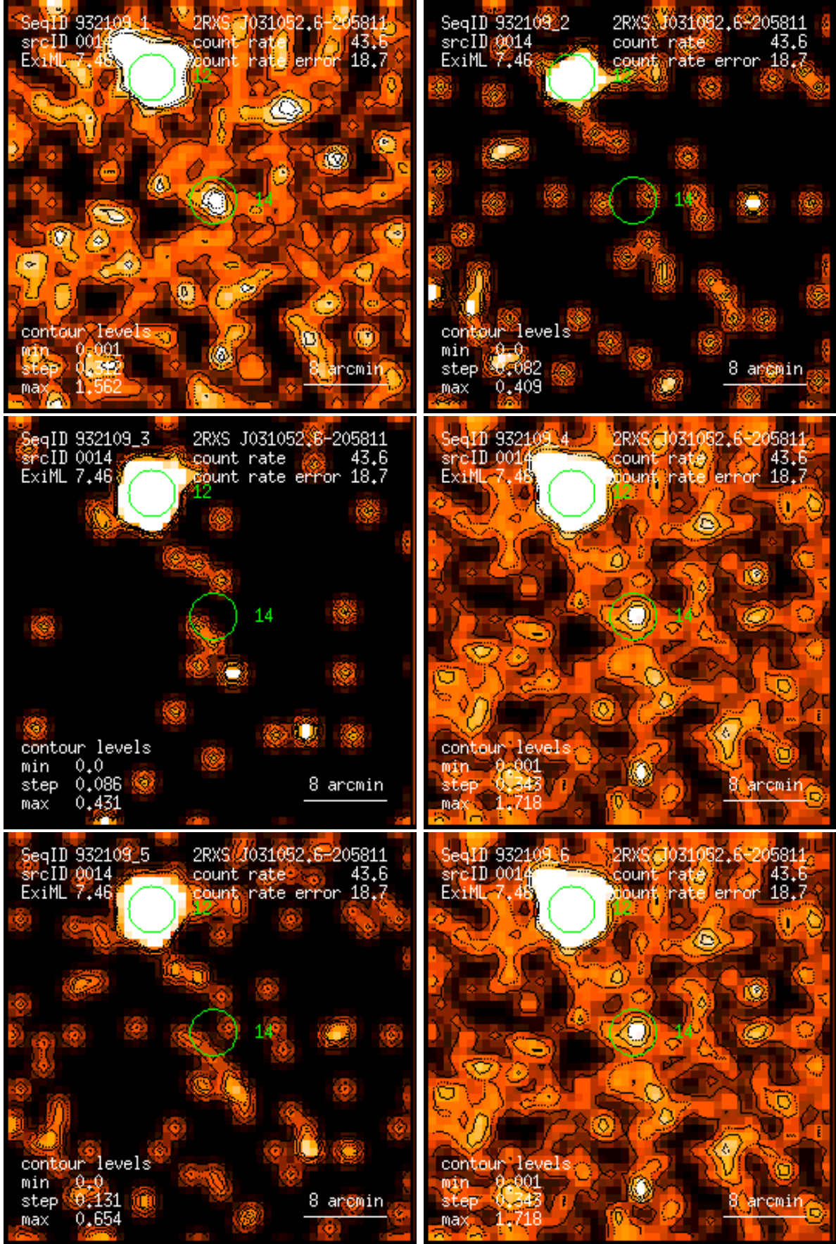
Figure 14: RASS 932109: detection 0014: band rate images, Gaussian filter: (1) PSPC channels 11 – 41, (2) 52 – 90, (3) 91 – 201, (4) 11 – 235, (5) 52 – 201, (6) 11 – 201. Broad band rates in counts/ks. Band rate contour levels in counts/ks/arcmin 2 .
