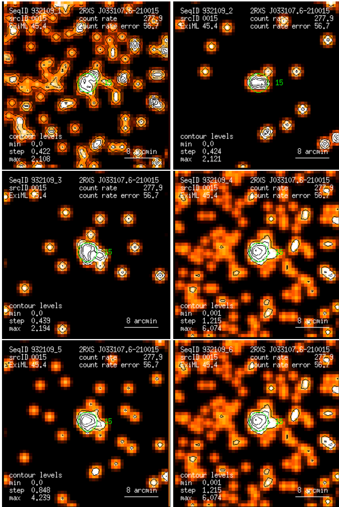
Figure 15: RASS 932109: detection 0015: band rate images, Gaussian filter: (1) PSPC channels 11 – 41, (2) 52 – 90, (3) 91 – 201, (4) 11 – 235, (5) 52 – 201, (6) 11 – 201. Broad band rates in counts/ks. Band rate contour levels in counts/ks/arcmin 2 .
