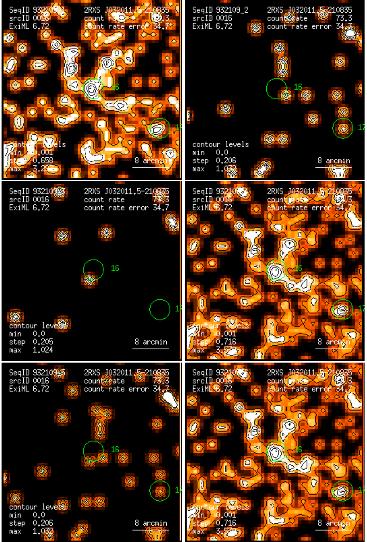
Figure 16: RASS 932109: detection 0016: band rate images, Gaussian filter: (1) PSPC channels 11 – 41, (2) 52 – 90, (3) 91 – 201, (4) 11 – 235, (5) 52 – 201, (6) 11 – 201. Broad band rates in counts/ks. Band rate contour levels in counts/ks/arcmin 2 .
