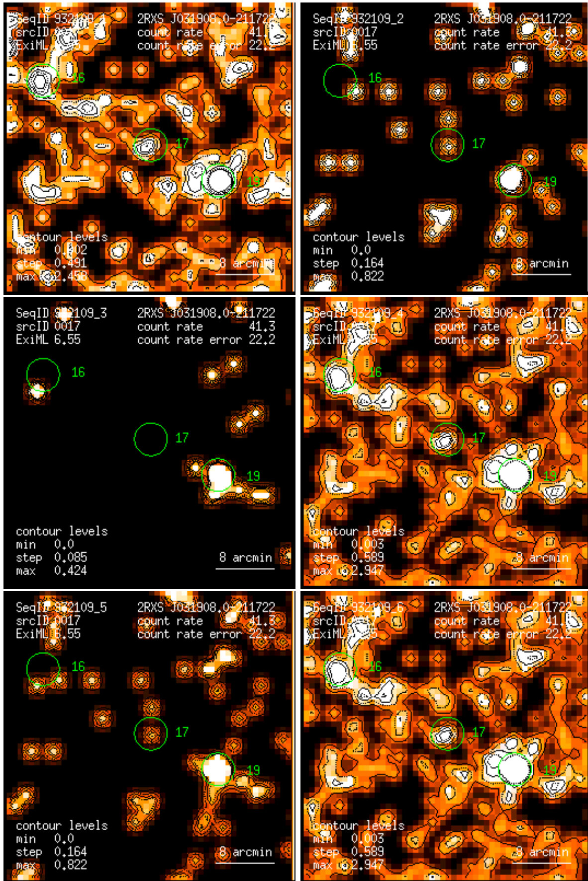
Figure 17: RASS 932109: detection 0017: band rate images, Gaussian filter: (1) PSPC channels 11 – 41, (2) 52 – 90, (3) 91 – 201, (4) 11 – 235, (5) 52 – 201, (6) 11 – 201. Broad band rates in counts/ks. Band rate contour levels in counts/ks/arcmin 2 .
