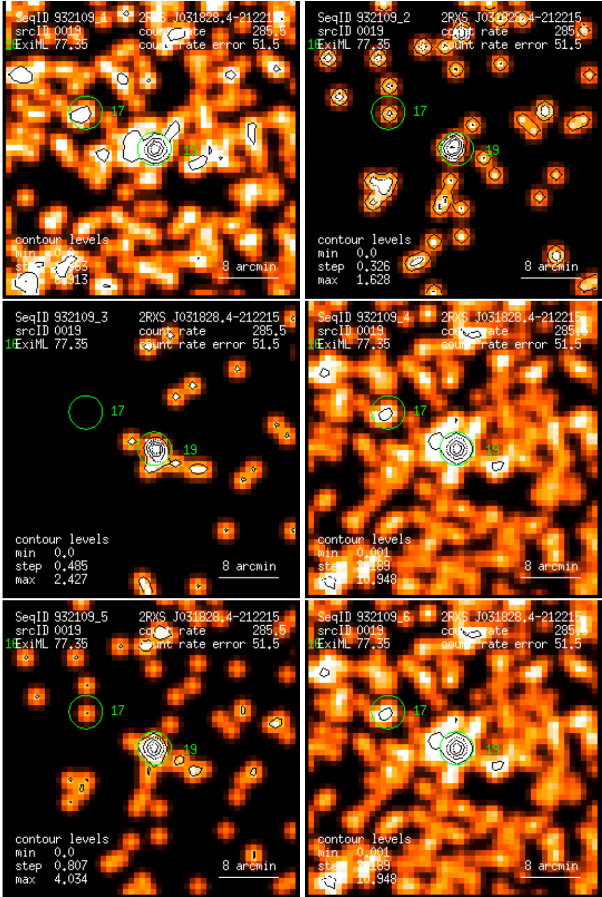
Figure 19: RASS 932109: detection 0019: band rate images, Gaussian filter: (1) PSPC channels 11 – 41, (2) 52 – 90, (3) 91 – 201, (4) 11 – 235, (5) 52 – 201, (6) 11 – 201. Broad band rates in counts/ks. Band rate contour levels in counts/ks/arcmin 2 .
