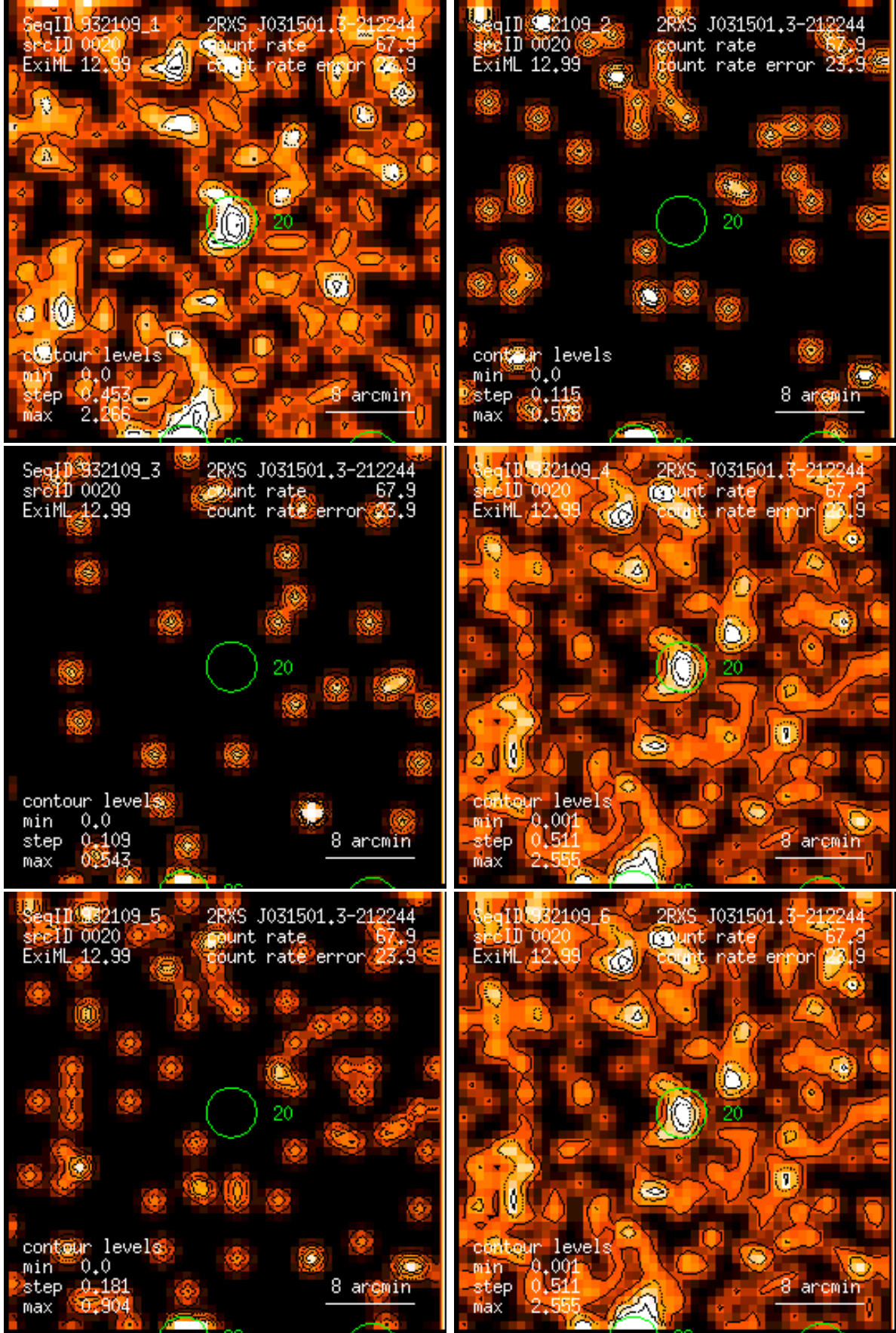
Figure 20: RASS 932109: detection 0020: band rate images, Gaussian filter: (1) PSPC channels 11 – 41, (2) 52 – 90, (3) 91 – 201, (4) 11 – 235, (5) 52 – 201, (6) 11 – 201. Broad band rates in counts/ks. Band rate contour levels in counts/ks/arcmin 2 .
