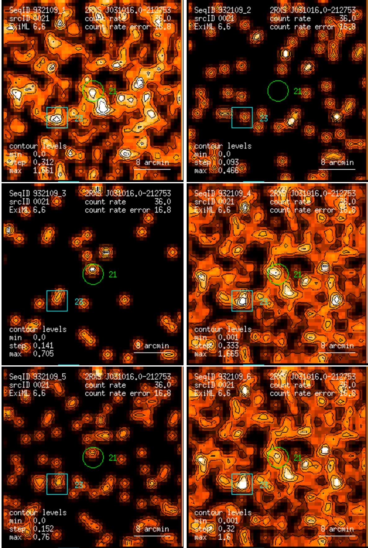
Figure 21: RASS 932109: detection 0021: band rate images, Gaussian filter: (1) PSPC channels 11 – 41, (2) 52 – 90, (3) 91 – 201, (4) 11 – 235, (5) 52 – 201, (6) 11 – 201. Broad band rates in counts/ks. Band rate contour levels in counts/ks/arcmin 2 .
