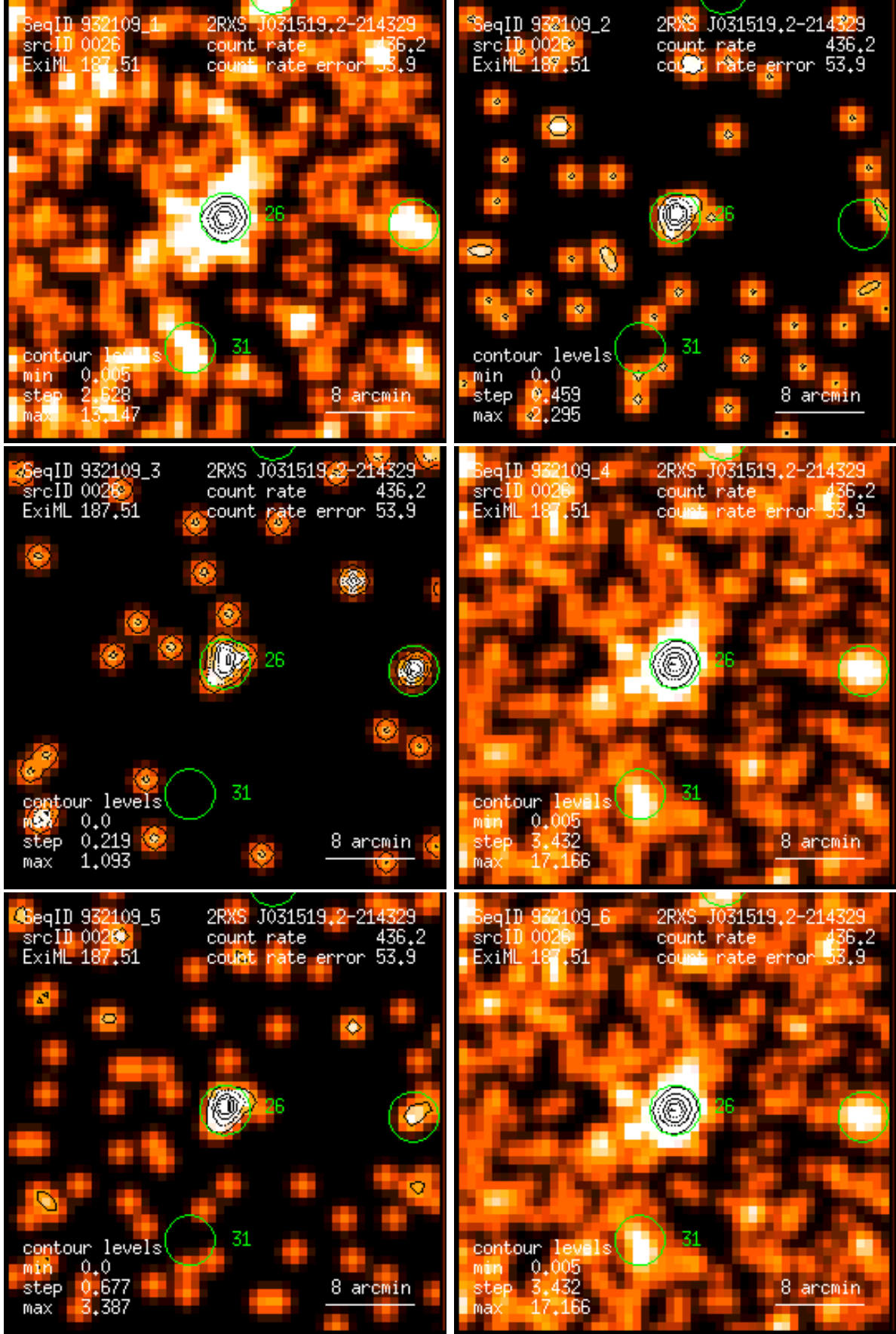
Figure 26: RASS 932109: detection 0026: band rate images, Gaussian filter: (1) PSPC channels 11 – 41, (2) 52 – 90, (3) 91 – 201, (4) 11 – 235, (5) 52 – 201, (6) 11 – 201. Broad band rates in counts/ks. Band rate contour levels in counts/ks/arcmin 2 .
