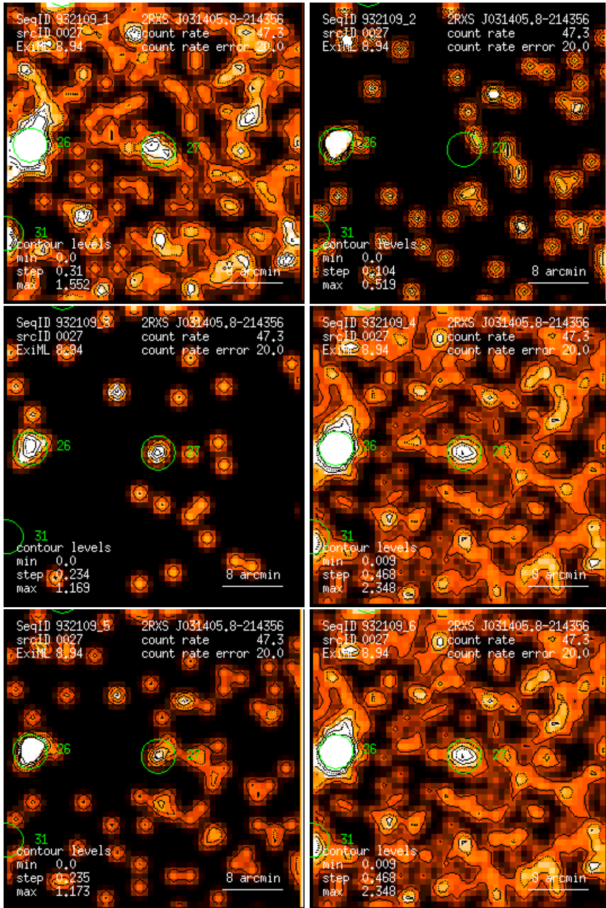
Figure 27: RASS 932109: detection 0027: band rate images, Gaussian filter: (1) PSPC channels 11 – 41, (2) 52 – 90, (3) 91 – 201, (4) 11 – 235, (5) 52 – 201, (6) 11 – 201. Broad band rates in counts/ks. Band rate contour levels in counts/ks/arcmin 2 .
