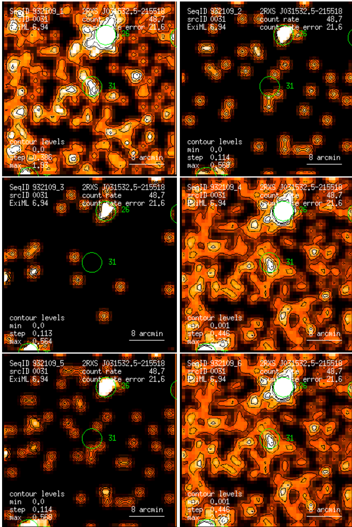
Figure 31: RASS 932109: detection 0031: band rate images, Gaussian filter: (1) PSPC channels 11 – 41, (2) 52 – 90, (3) 91 – 201, (4) 11 – 235, (5) 52 – 201, (6) 11 – 201. Broad band rates in counts/ks. Band rate contour levels in counts/ks/arcmin 2 .
